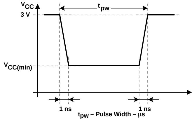
Figure 16. V_{CC(min)} Level With a Square Voltage Drop to Generate a POR/Brownout Signal
