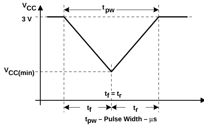
Figure 17. V_{CC(min)} Level With a Triangle Voltage Drop to Generate a POR/Brownout Signal
