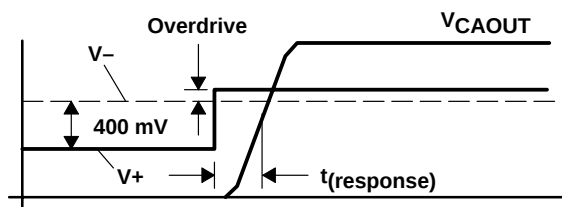
Figure 14. Overdrive Definition
