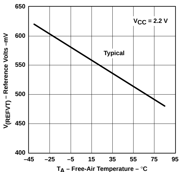
Figure 12. V(REFVT) vs Temperature, VCC = 2.2 V
