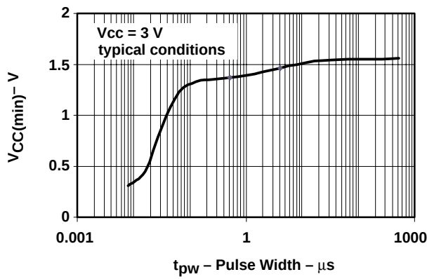
Figure 16. V_{CC(min)} Level With a Square Voltage Drop to Generate a POR/Brownout Signal
