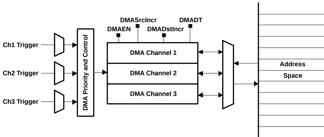
Figure 1. Block Diagram Direct Memory Access (DMA)
