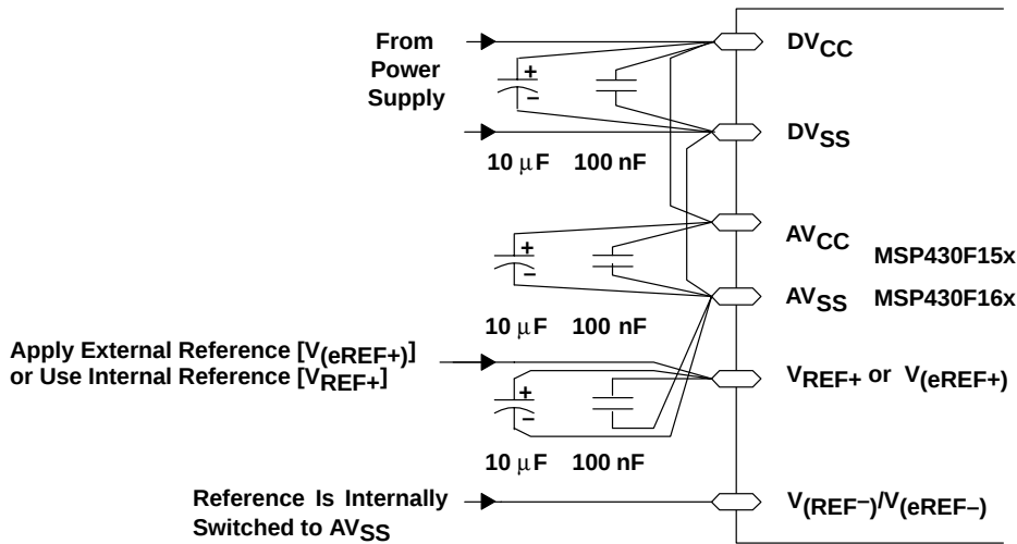
Figure 23. Supply Voltage and Reference Voltage Design V_{(REF-)/V(eREF-)} = AVSS , Internally Connected
