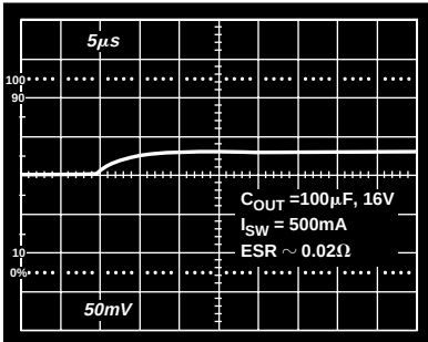
Figure 14. OS-CON Capacitor
