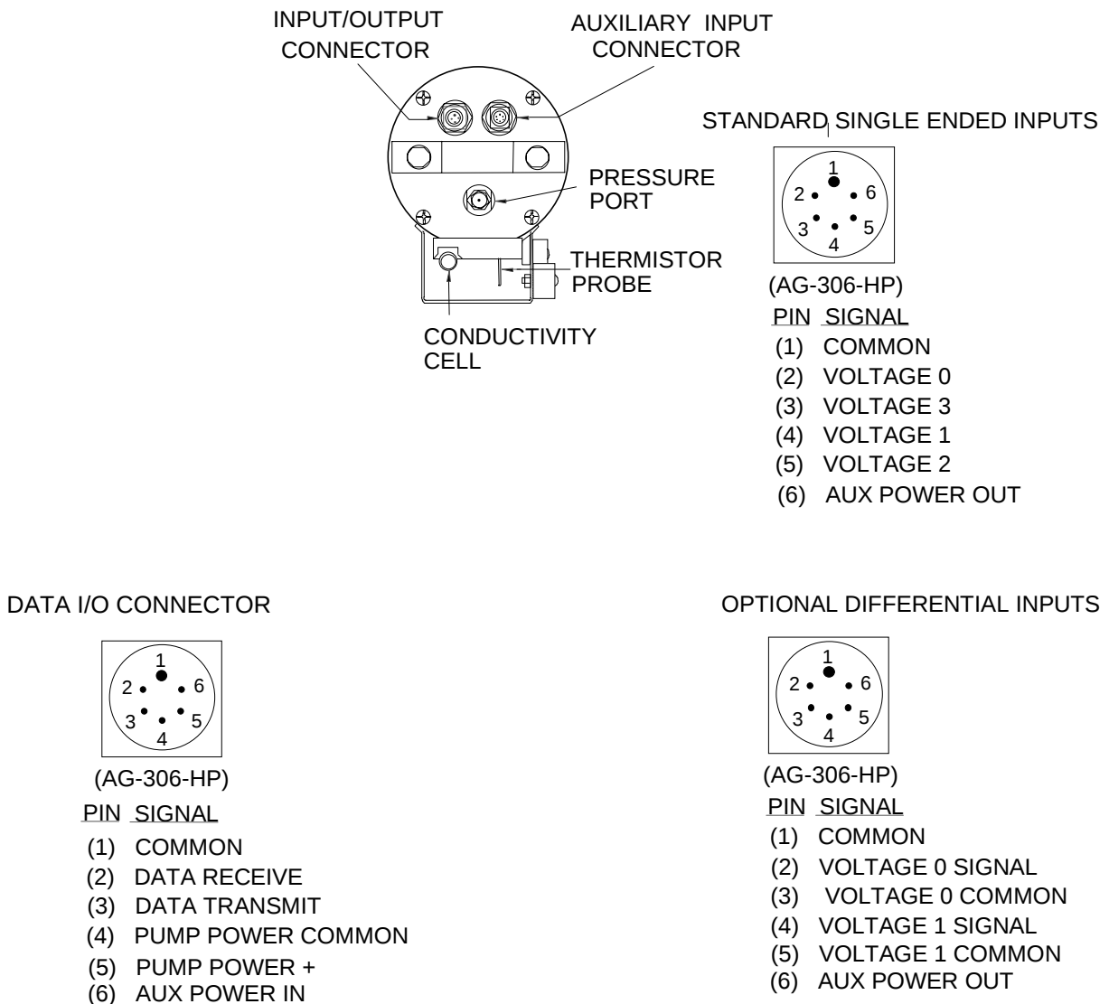
Figure 1 Connector Congurations for the SEACAT Profiler.
