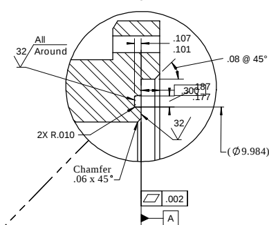
DETAIL B SCALE 1 : 1 O-Ring 2-274
