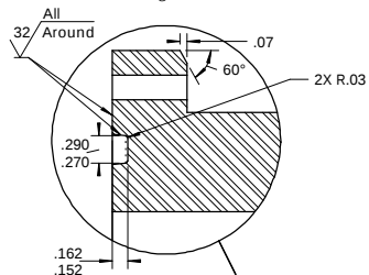
DETAIL C SCALE 1 : 1 O-Ring 2-378
