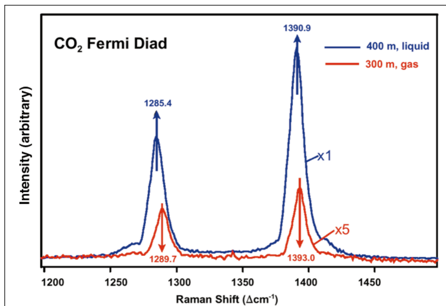
FIG. 7. Raman spectra of liquid and gaseous \text{CO}_2 collected during small-scale \text{CO}_2 injection experiments on the ROV Tiburon. Raman spectra were acquired during ascent from the ocean floor while DORISS was sitting in the ROV's toolshed. Difference in phase is recognized by strong increase in intensity and spectral downshift in the liquid compared to the gas. In this figure, the peak positions are uncorrected for depth-induced wavenumber shifts. The spectral separation between the two \text{CO}_2 peaks (more accurately measurable than the absolute peak positions) is shown in Fig. 8.
