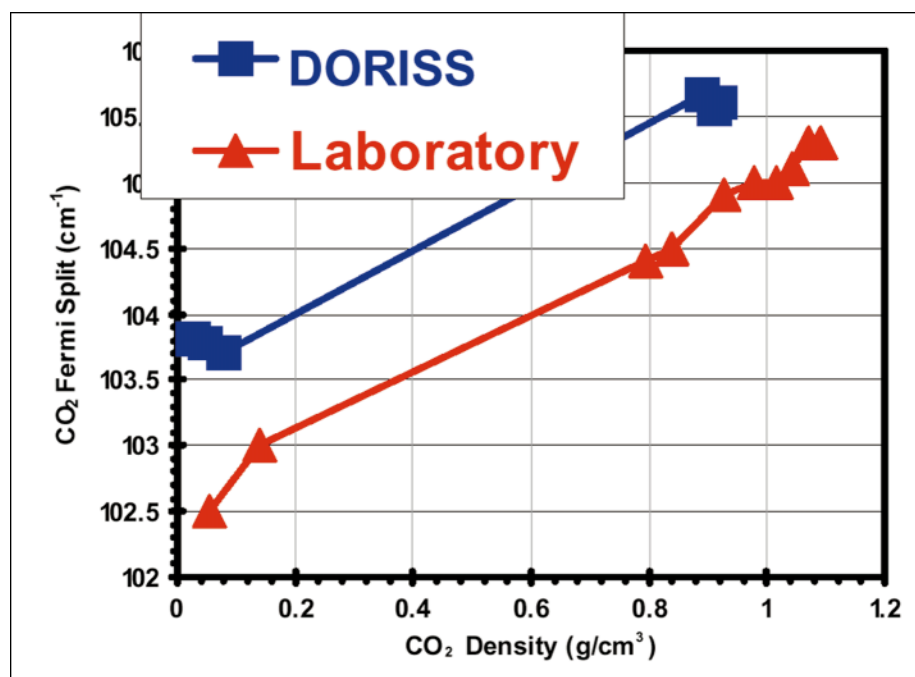
Fig. 8. Plot of the Raman spectral separation between the two peaks of Fermi diad of CO 2 versus CO 2 density (see text). Laboratory data were collected at 23 °C at well-calibrated pressures; Raman peak positions were corrected based on gas emission lines from calibration lamps. 22 DORISS data (uncorrected peak positions) were collected in ascent from 664 m depth in the ocean. Parallelism of laboratory and DORISS data indicates appropriate spectral response to changes in density. Offset between the two curves suggests that the dispersion function that was applied to the DORISS was inappropriate under the specific dive conditions.
