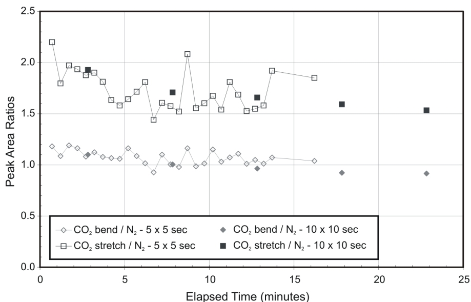
Figure 7. Peak area ratios over time from the August 2002 gas cube experiment. Data points are plotted at the midpoint of the accumulation time.
