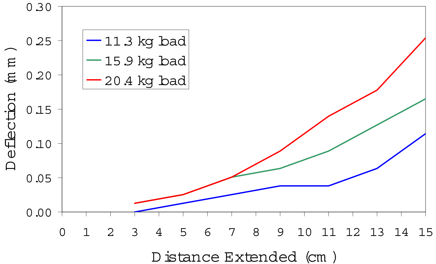
PUP Deflection Plot
