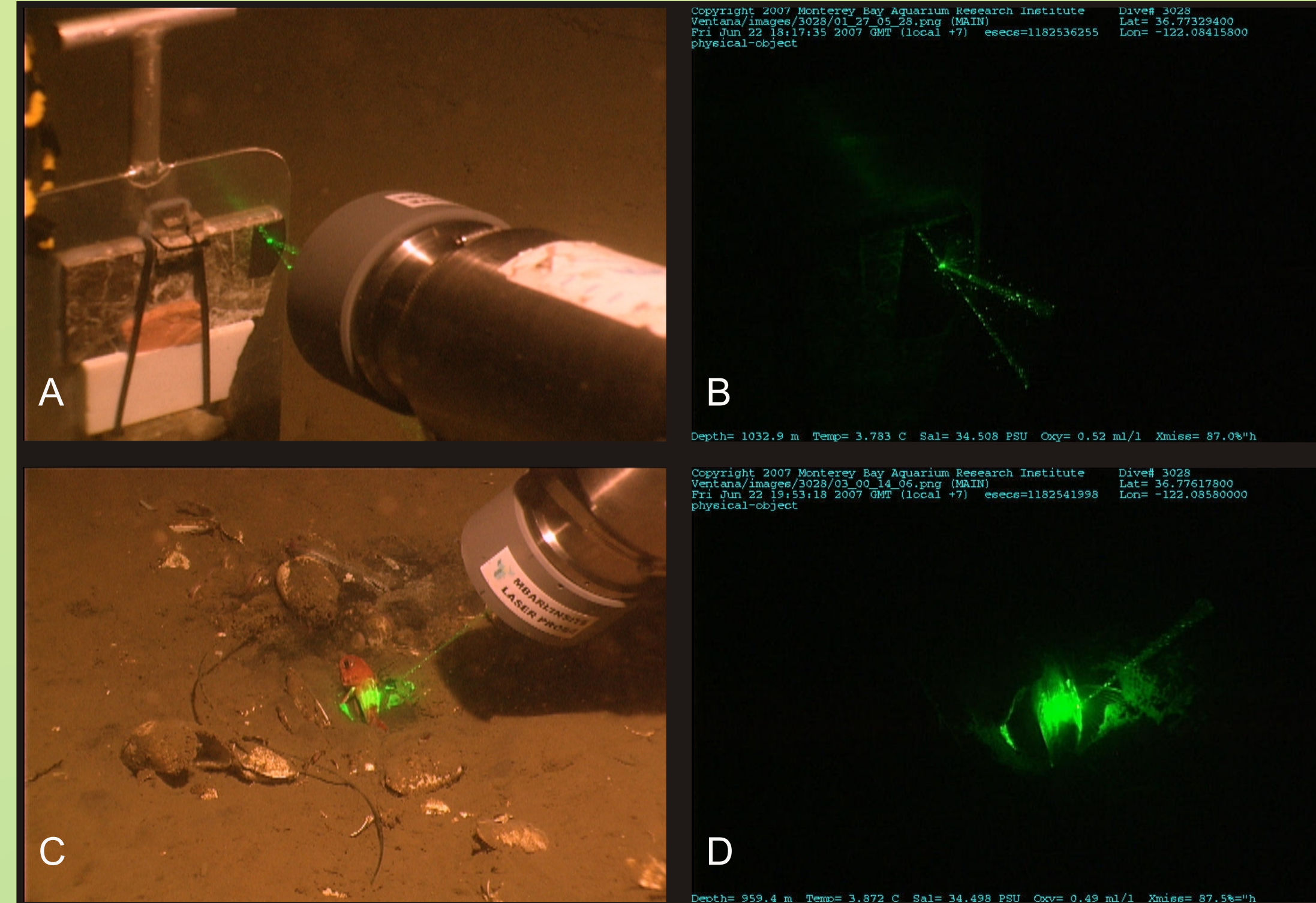
Figure 4. (A) Laser Raman probehead is approaching the silicon wafer specimen on the target tray. In this view the target tray is sitting upright on the sea-floor detached from the ROV to test the effect of ROV vibrations on spectra obtained while the probehead is held in the manipulator grip. (B) Same as figure A but with the ROV lights off so that a Raman spectrum can be collected without interference from the ROV lights. (C) Laser Raman probehead approaching a rockfish on the sea-floor. (D) Same as figure C but again with the ROV lights off.
