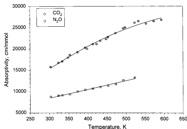
Figure 2. The absorptivity of \text{CO}_2 and \text{N}_2\text{O} in \text{H}_2\text{O} (275 bar) as a function of temperature.
