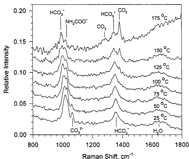
Figure 3. FT-Raman spectra of 1.2 m (\text{NH}_4)_2\text{CO}_3 at 275 bar as a function of temperature showing the components of Scheme 2.
