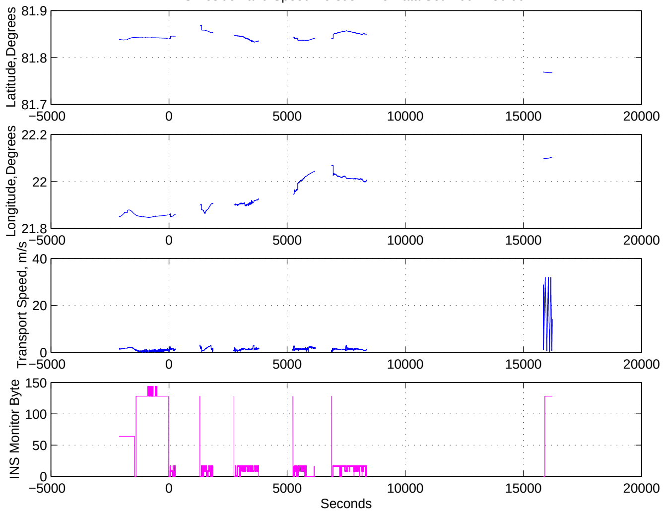
INS Position and Speed Versus Time Data Set: 2001.286.00
