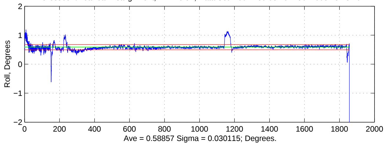
Crossbow/Kearfott Misalignment; 2-1 Euler ; Data Set: 2001.289.03 25-Feb-2003 15:18:10
