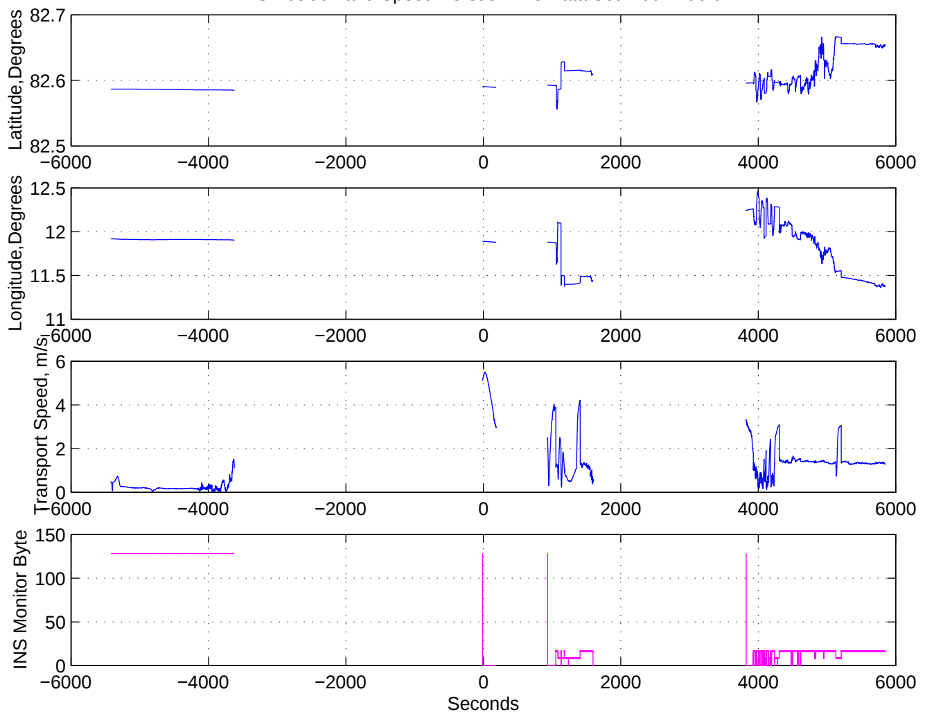
INS Position and Speed Versus Time Data Set: 2001.290.04
