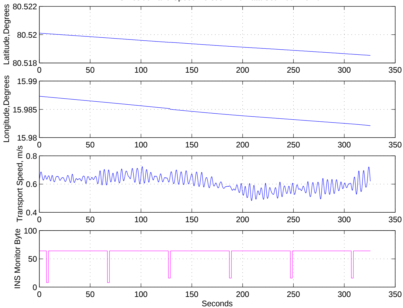
INS Position and Speed Versus Time Data Set: 2001.297.02
