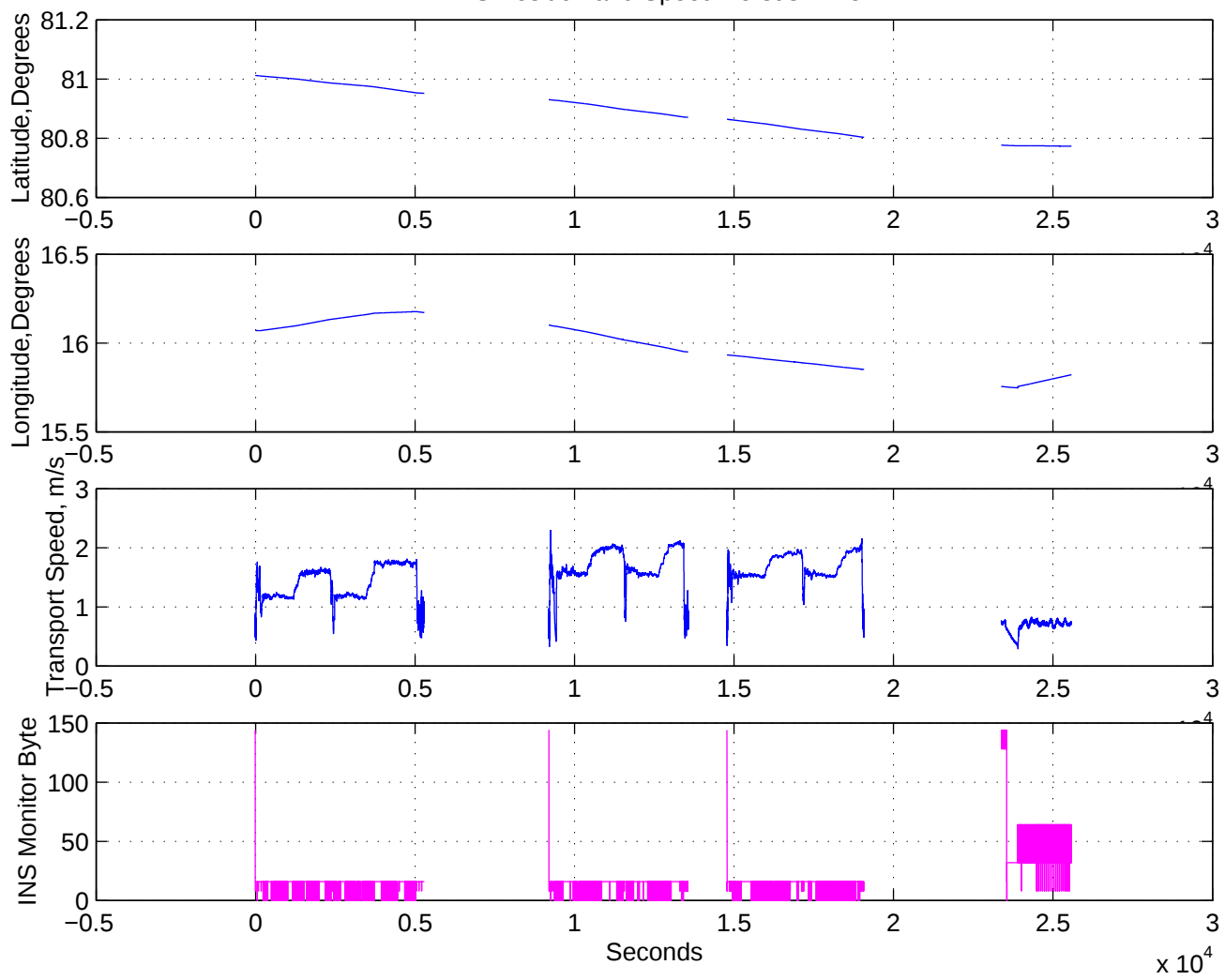
INS Position and Speed Versus Time
