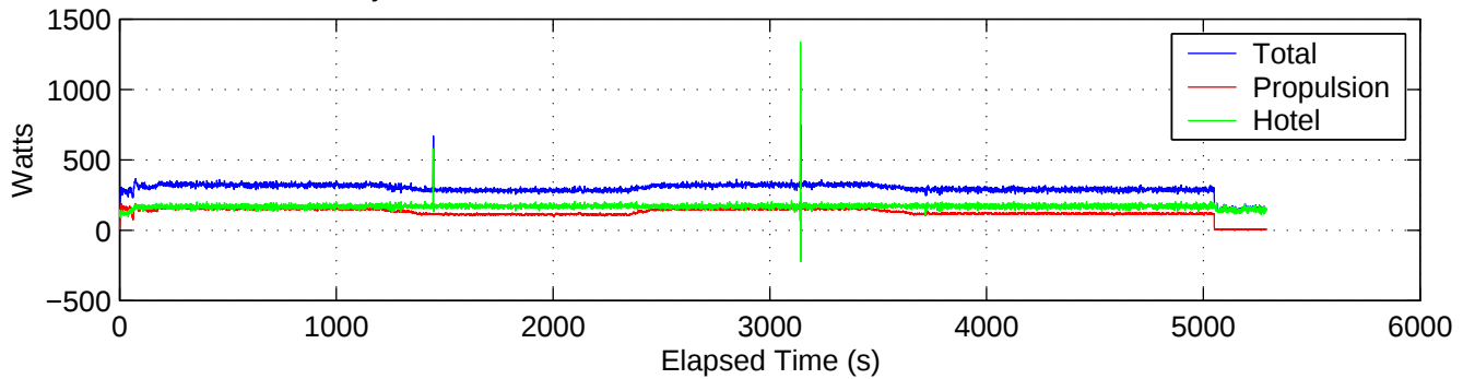
Metrabyte Power ; Data Set: 2001.297.03 Plotted on 28-Feb-2003 16:17:21
