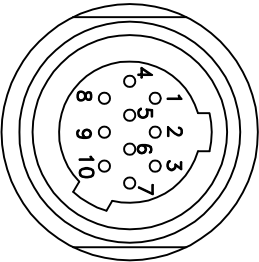
MINK-10-BCR CONNECTOR FACE VIEW
