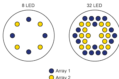
Multiray LSL-2025 LED Array Layout
