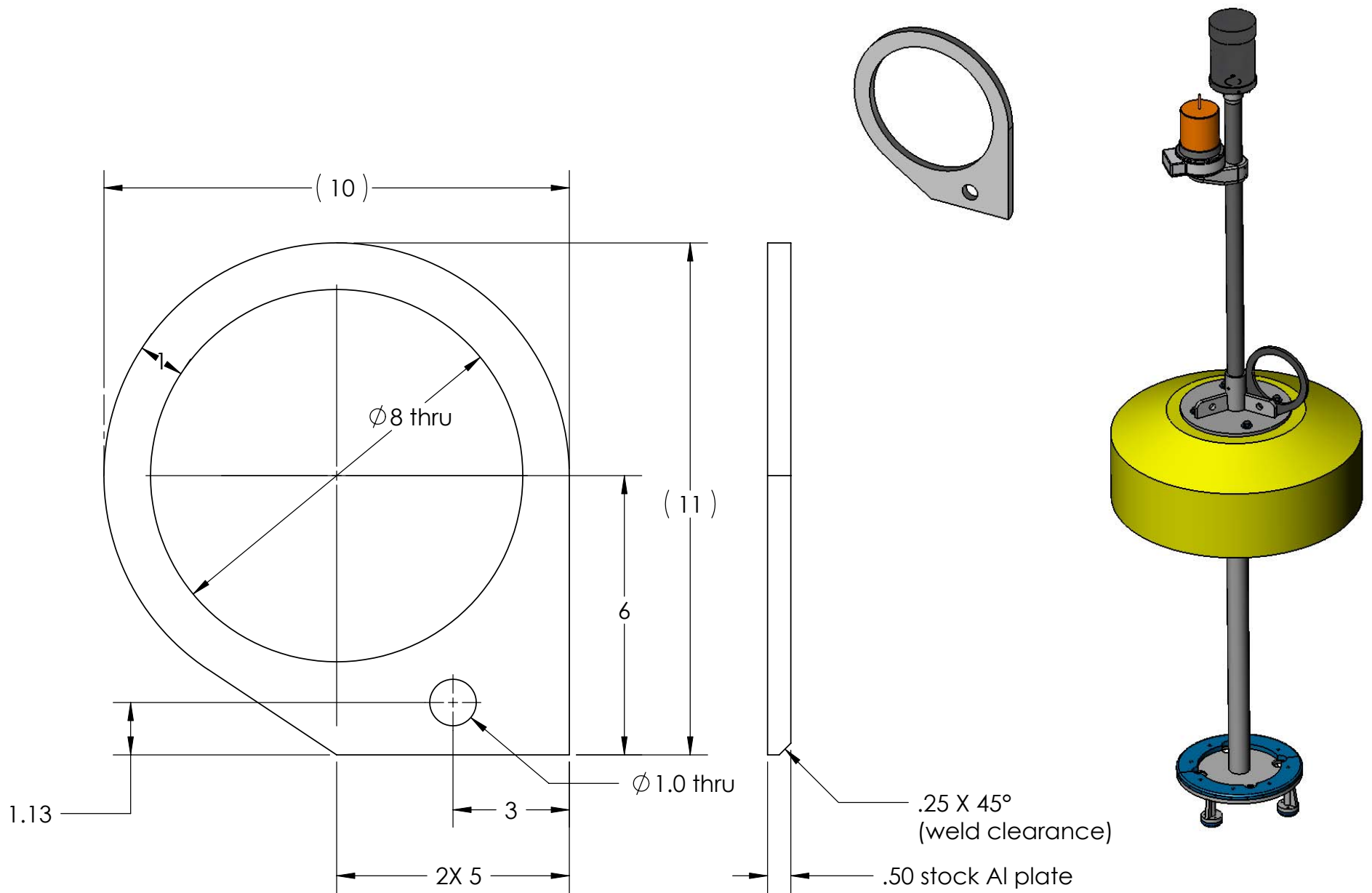
LOBO Moring Lift Ring Waterjetted out of 1/2" 6061 Al plate Hans Jannasch, 5/20/08
