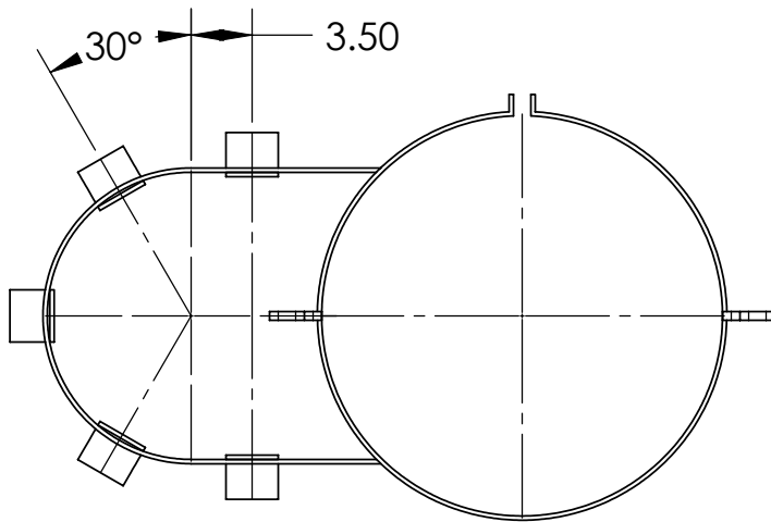
Welded Assembly
