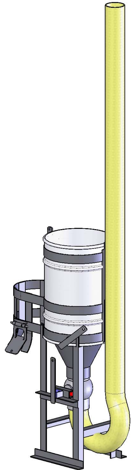
CORK-top cement barrel concept Hans Jannasch, MBARI, 8/10/07
