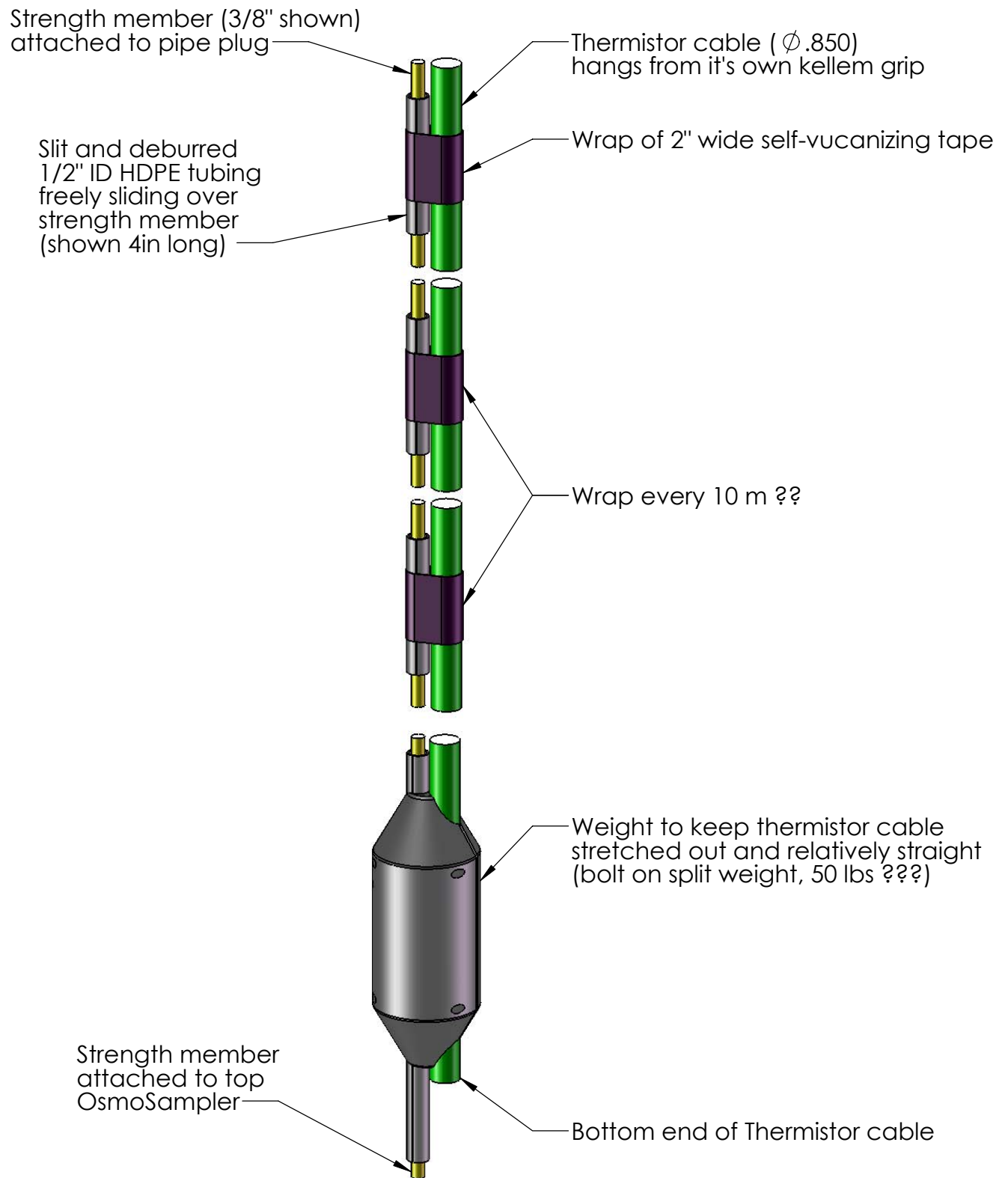
Free-hanging Thermistor String Concept
