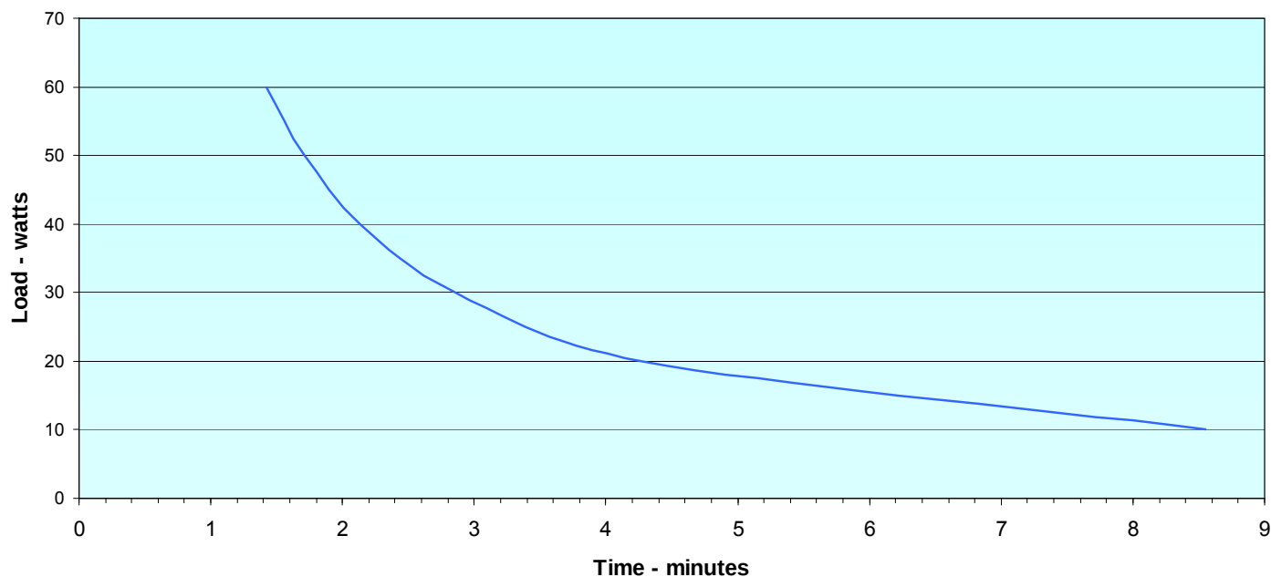
BAT-SC350 Hold-up Time
