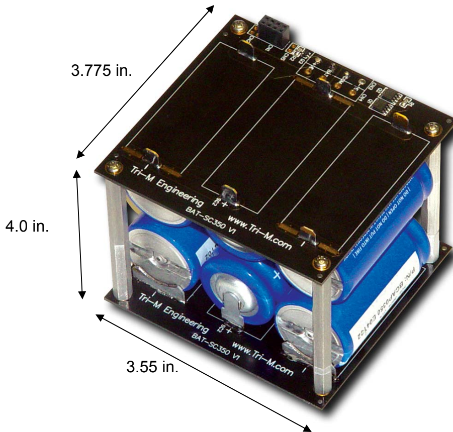
Figure 1 - CBP58 Dimensions
