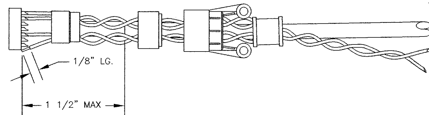
"DETAIL A"
