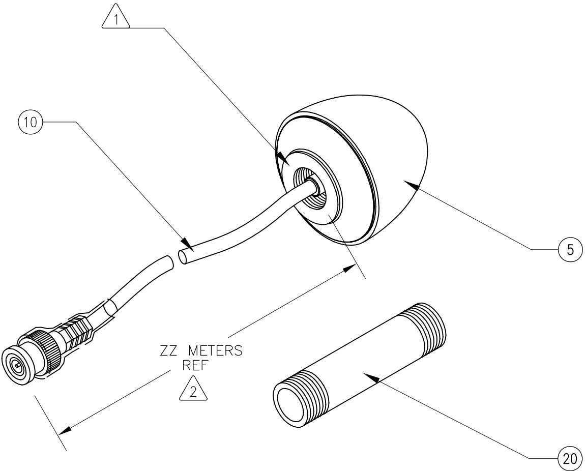
ISOMETRIC VIEW
