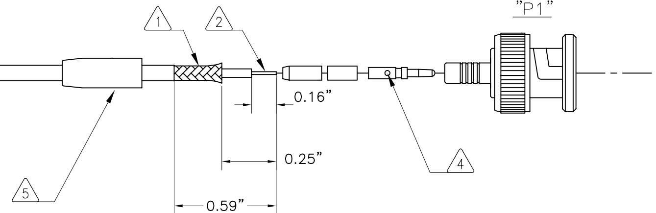
"DETAIL B"
