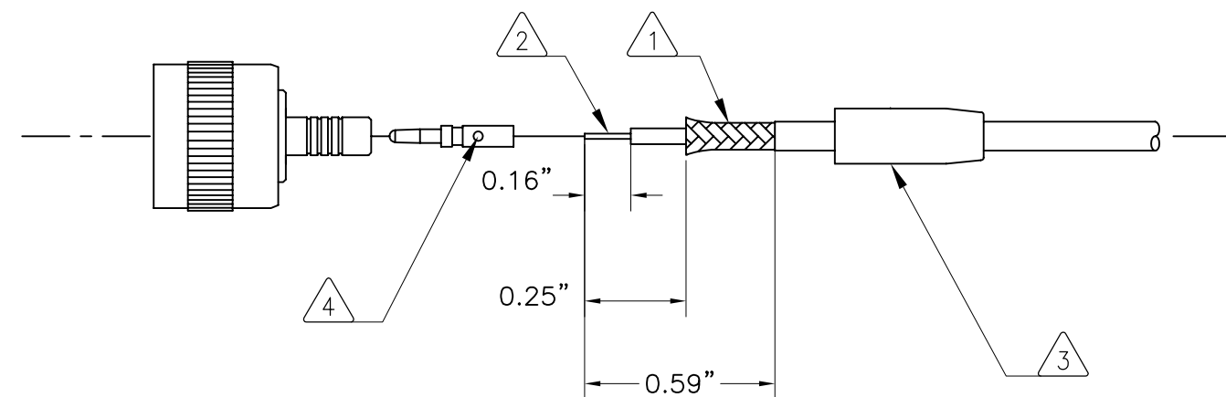
"DETAIL A"
