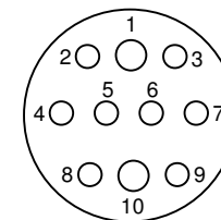
MINK-10-CCPL SOCKETS, FACE VIEW
