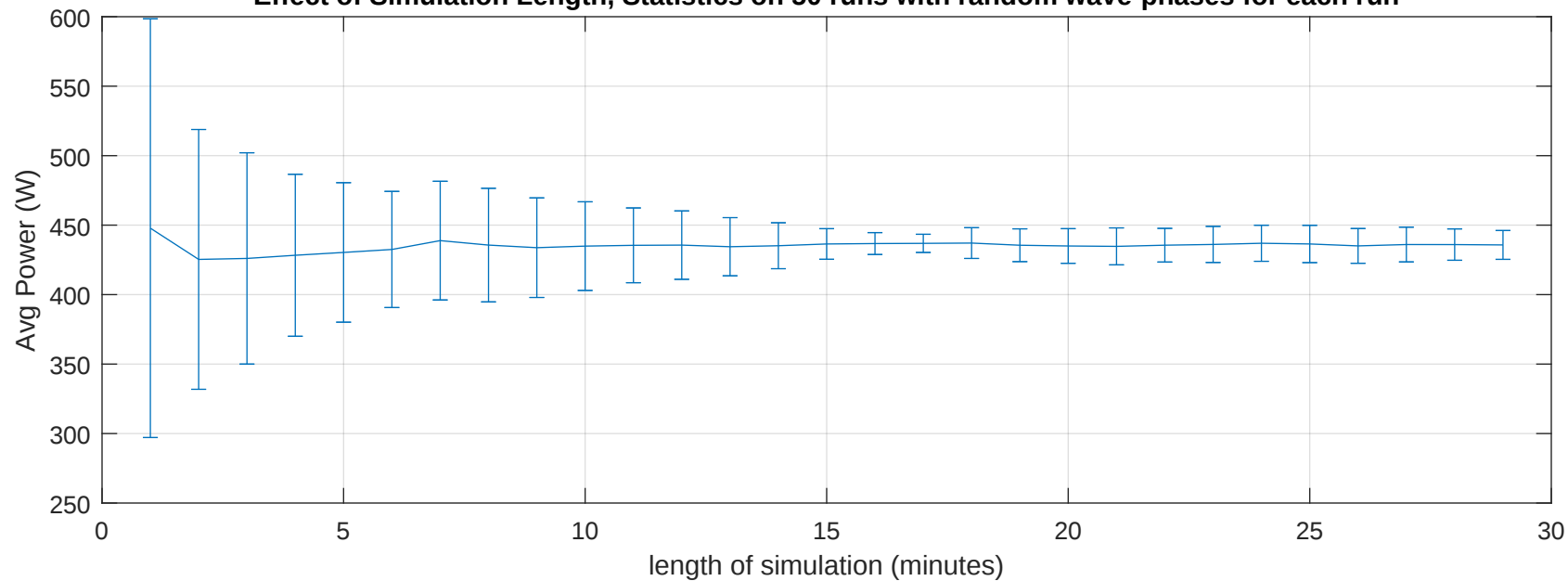
Effect of Simulation Length, Statistics on 50 runs with random wave-phases for each run
