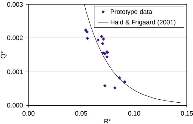
Fig. 6. Comparison of preliminary prototype data [2,4] and overtopping expression.
