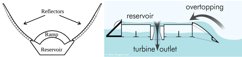
Fig. 1. Left : Main components of the Wave Dragon. Right : The basic principle of the Wave Dragon: (1) waves overtopping a ramp, (2) water stored in a reservoir above sea level and (3) water discharged through hydro turbines. Wave Dragon floats on open air-chambers used to adjust floating level.
