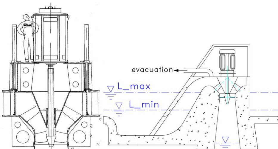
Fig. 5. Cylinder gate on/off turbine (left) and siphon type on/off turbine.
