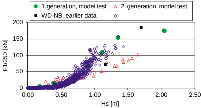
Fig. 7. Comparison of mooring forces in terms of F_{1/250} (average of the 1/250 largest peaks) measured during model tests [5] and prototype measurements in Nissum Bredning (WD-NB) [12]. Results are given in prototype scale.
