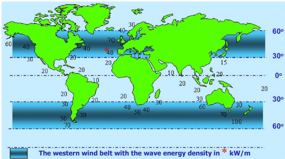
Fig. 3. World distribution of average wave energy (kW/m).
