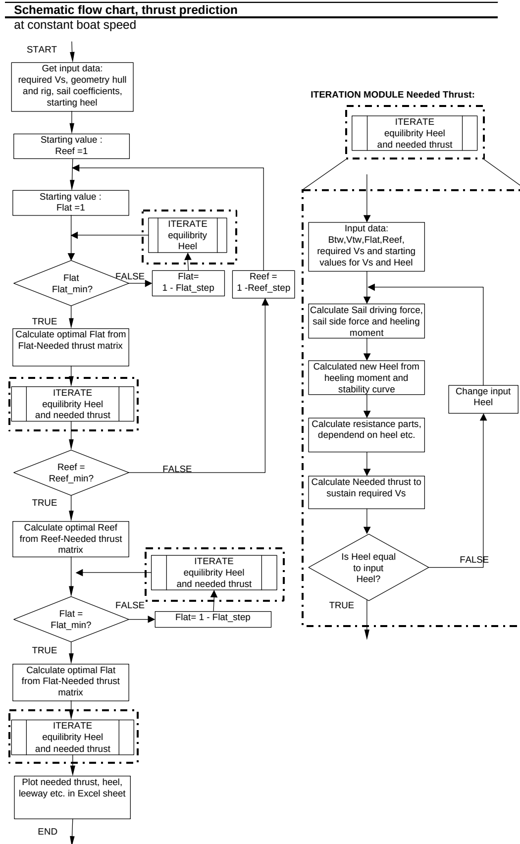
Figure 2 Schematic flow chart of the TPP
