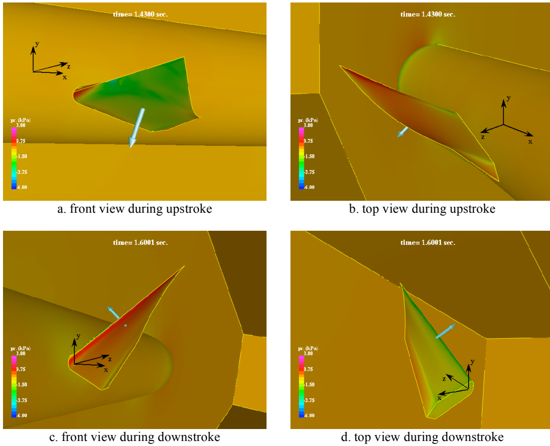
Figure. 16. Pressure distribution on the fin at maximum thrust production instants.
