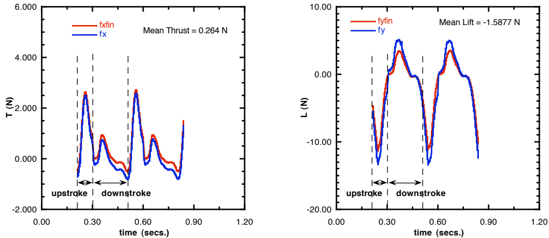
Figure 10. Thrust and Lift production for a UUV moving at 3kts, \alpha_r = 10^\circ , \phi_{\max} = 114^\circ , f = 3.333\text{Hz} .
