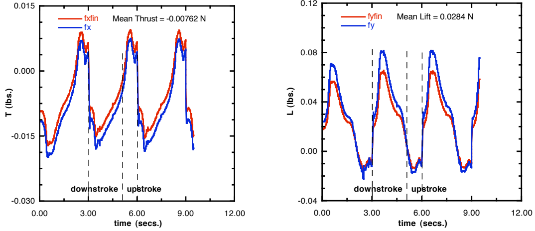
Figure 4. Thrust and Lift production for a hovering UUV, f = 0.333\text{Hz} .
