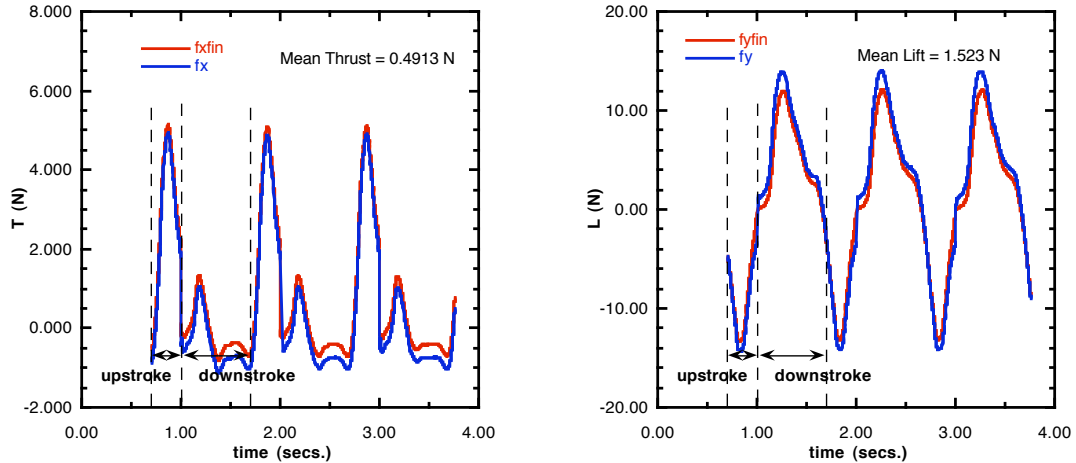
Figure. 13. Thrust and Lift production for a UUV moving at 3kts, \alpha_r = 20^\circ , \phi_{\max} = 114^\circ , f = 1.0\text{Hz} , rib spacing of 2cm and with doubled rib lengths.
