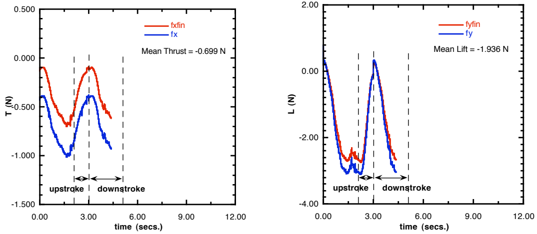
Figure 7. Thrust and Lift production for a UUV moving at 3kts, \alpha_r = 0^\circ , f = 0.333\text{Hz} .
