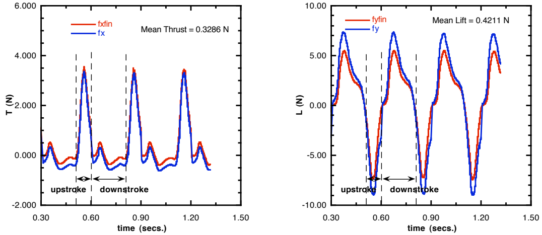
Figure. 12. Thrust and Lift production for a UUV moving at 3kts, \alpha_r = 20^\circ , \phi_{\max} = 114^\circ , f = 3.333\text{Hz} .
