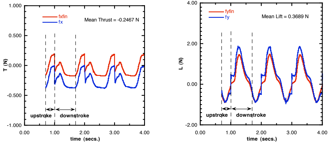
Figure. 11. Thrust and Lift production for a UUV moving at 3kts, \alpha_r = 20^\circ , \phi_{\max} = 114^\circ , f = 1.0\text{Hz} .
