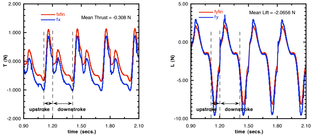
Figure 8. Thrust and Lift production for a UUV moving at 3kts, \alpha_r = 0^\circ , f = 3.333\text{Hz} .
