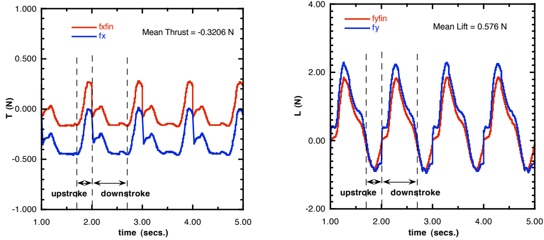
Figure. 14. Thrust and Lift production for a UUV moving at 3kts, \alpha_r = 20^\circ , \phi_{\max} = 114^\circ , f = 1.0\text{Hz} , rib spacing = 1.2cm and with original rib lengths.
