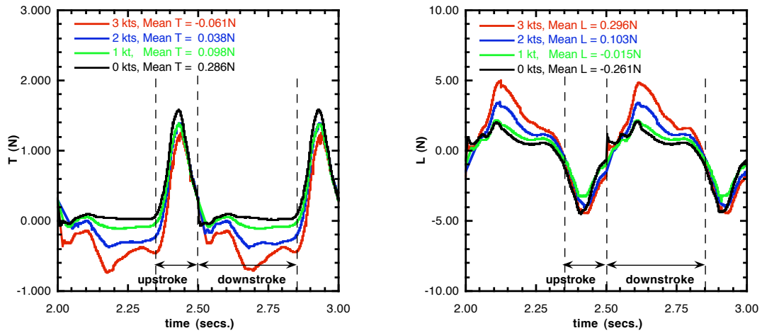
Figure 18. Effect of inflow velocity on the thrust and lift production, f = 2.0\text{ Hz} .
