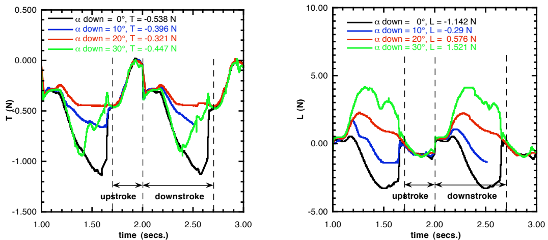
Figure 20. Effect of angle of attack during the downstroke on force production, f = 1\text{ Hz} .
