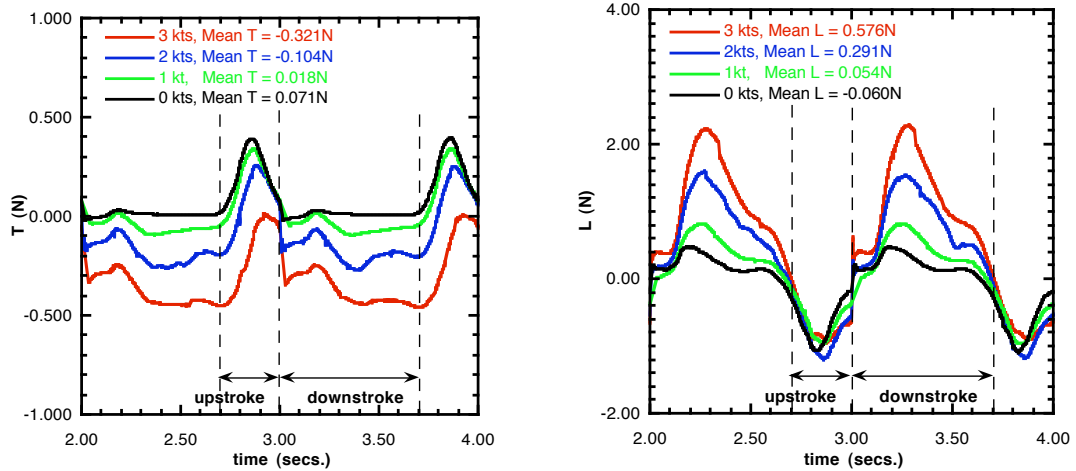
Figure 19. Effect of inflow velocity on the thrust and lift production, f = 1.0\text{ Hz} .
