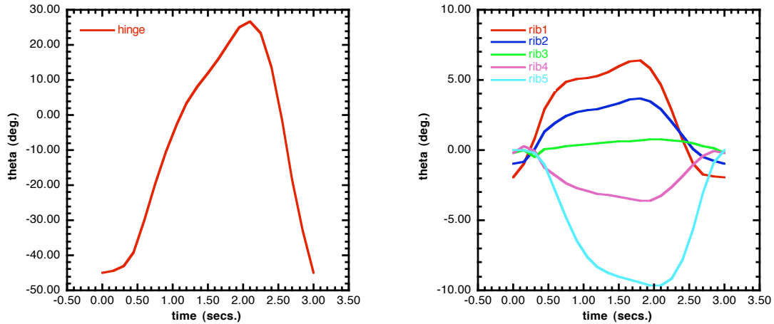
Figure 3. Rotation of the hinge and the additional rotation of the ribs, f = 3.333\text{Hz} .
