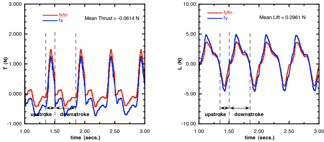
Figure. 15. Thrust and Lift production for a UUV moving at 3kts, \alpha_r = 20^\circ , \phi_{\max} = 114^\circ , f = 2.0\text{Hz} , rib spacing = 1.2cm and with original rib lengths.
