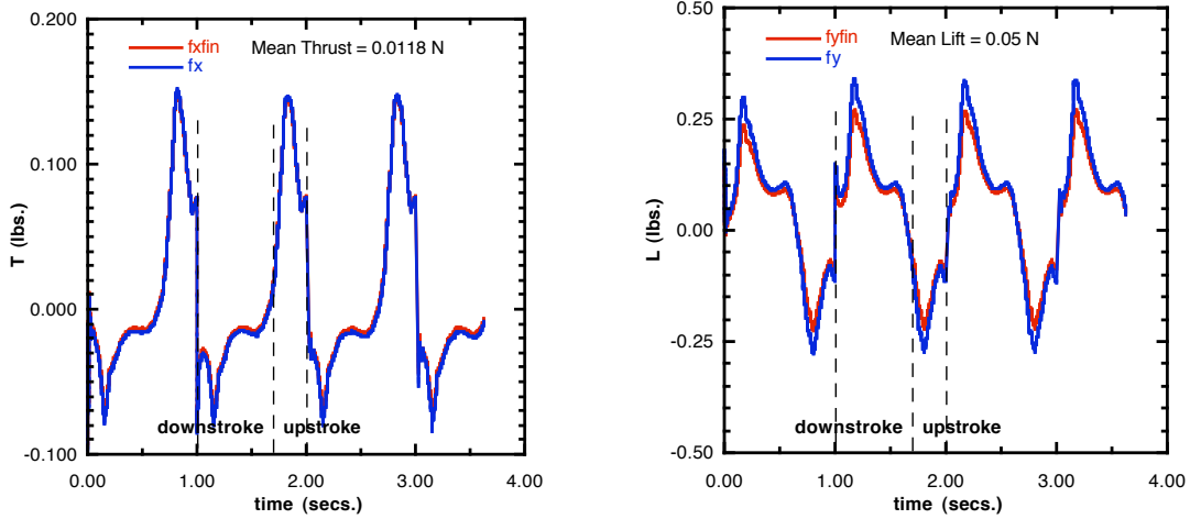
Figure 5. Thrust and Lift production for a hovering UUV, f = 1.0\text{Hz} .
