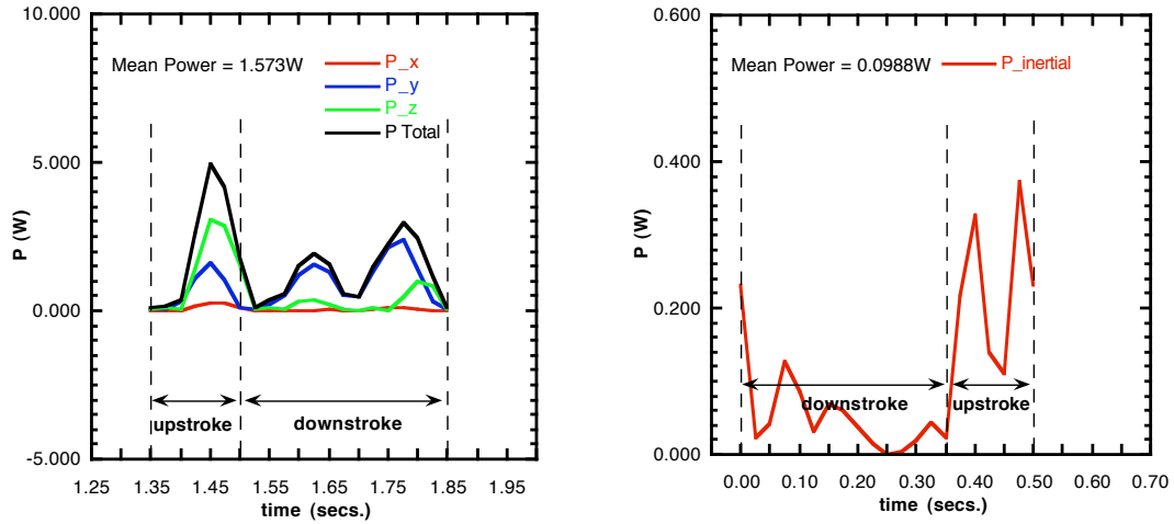
Figure. 17. Power requirement for moving the fin for a UUV moving at V = 3\text{kts} , f = 2.0\text{Hz} , (a) Hydrodynamic, (b) Inertial.
