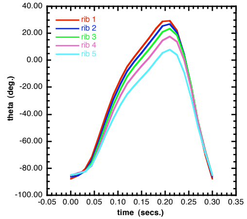
Figure 9. Rotations of the ribs for increased amplitude, f = 3.333\text{Hz} .
