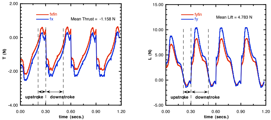
Figure 6. Thrust and Lift production for a UUV moving at 3kts, f = 3.333\text{Hz} .
