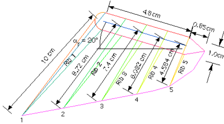
Figure 2. Schematic of the deforming fin showing the root cross-section and the 5 ribs.
