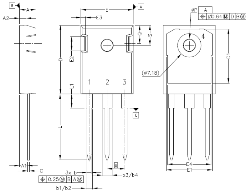
Package TO-247-3
