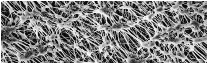
Gore's ePTFE membrane magnified 40,000 times.
