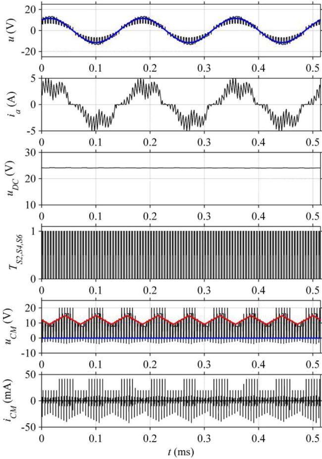
Fig. 5. Simulation results of the HCBB with the synchronous modulation scheme L_{1,2,3} = 3.3 \mu\text{H} . Generator back EMF u_{\text{emf},a} (blue) and terminal voltage u_{t,a} (black), phase current i_a , output voltage u_{\text{DC}} , switching signals for the three-phase legs T_{S2}, S4, S6 , as well as CM voltage u_{\text{CM}} [including the envelope, cf. (9) and (10)] and current i_{\text{CM}} , are shown. The switching frequency is f_s = 200 \text{ kHz} , and the fundamental frequency is f_f = 5833 \text{ Hz} (350 000 r/min), whereas C_{Y-\text{GND}} was assumed to be 48 pF (cf. Fig. 7).
