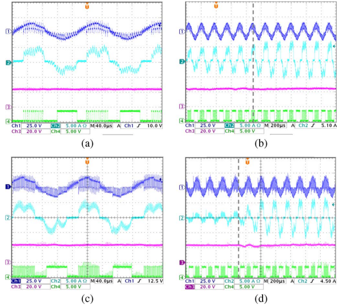
Fig. 17. Measurement results of the HCBR with the sector detection modulation scheme at 350 000 r/min, switching frequencies of (a)/(b) f_s = 200 kHz and (c)/(d) f_s = 400 kHz, and output power of (a)/(c) 50 W, as well as (dashed vertical line) output power step changes of (b) from 30 to 60 W and (d) from 15 to 75 W. (Channel 1) Terminal voltage. (Channel 2) Phase current. (Channel 3) Output voltage. (Channel 4) PWM signal for one switch.
