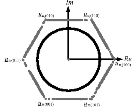
Fig. 6. Simulation of space vectors for the HCBB for the synchronous modulation scheme. (Black) Back EMF. (Gray) Terminal voltage.
