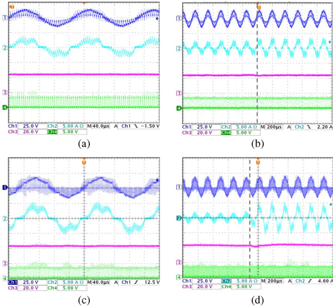
Fig. 16. Measurement results of the HCBR with the synchronous modulation scheme at 350 000 r/min, switching frequencies of (a)/(b) f_s = 200 kHz and (c)/(d) f_s = 400 kHz, and output power values of (a) 40 W and (c) 50 W, as well as (dashed vertical line) output power step changes of (b) from 15 to 40 W and (d) from 15 to 50 W. (Channel 1) Terminal voltage. (Channel 2) Phase current. (Channel 3) Output voltage. (Channel 4) PWM signal for all three switches.
