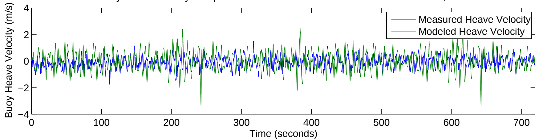
Buoy Heave Velocity Comparison – Measurements and Sea State from Feb 11, 2011
