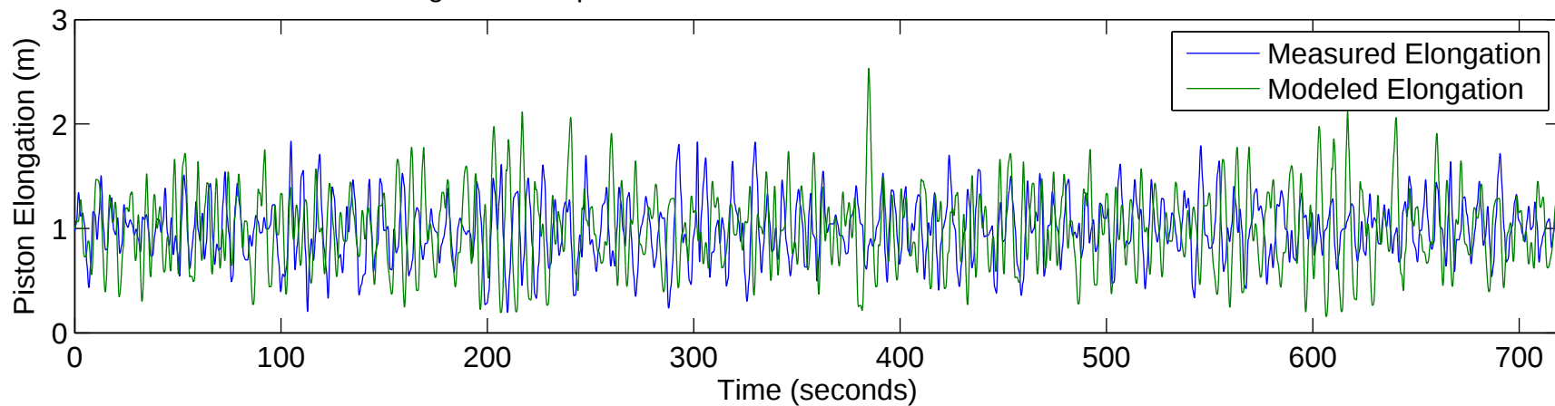
PTO Elongation Comparison – Measurements and Sea State from Feb 11, 2011
