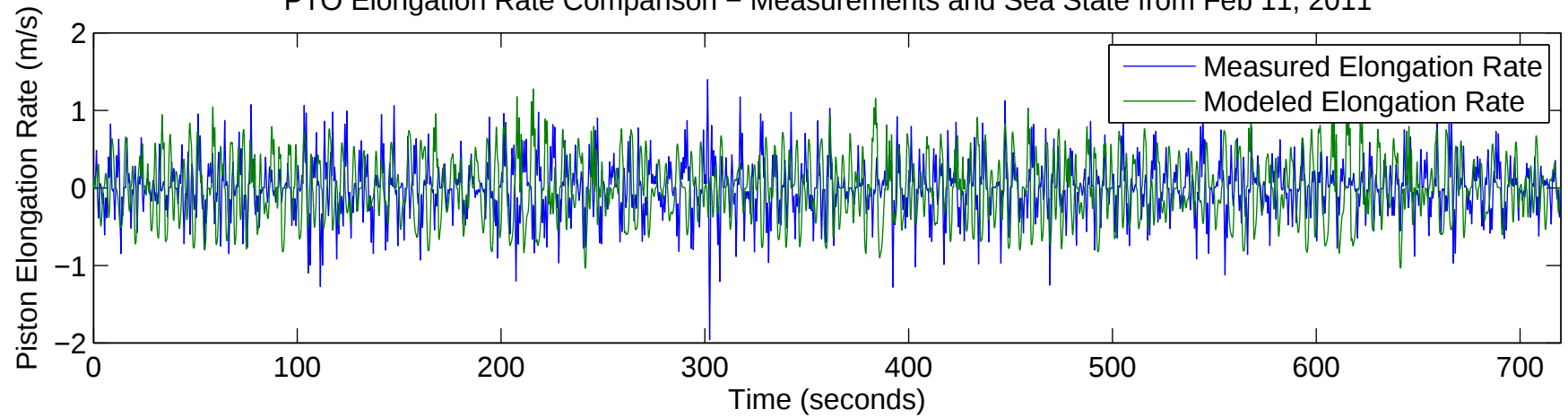
PTO Elongation Rate Comparison – Measurements and Sea State from Feb 11, 2011
