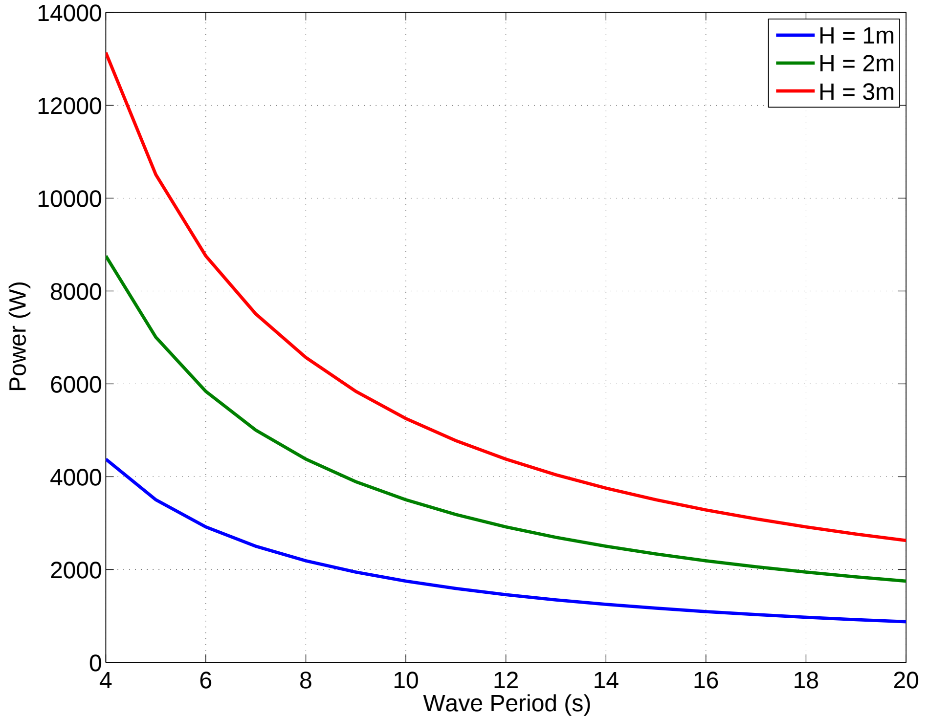
Upper bound for 5000 lb displacement point absorber in heave – regular waves
