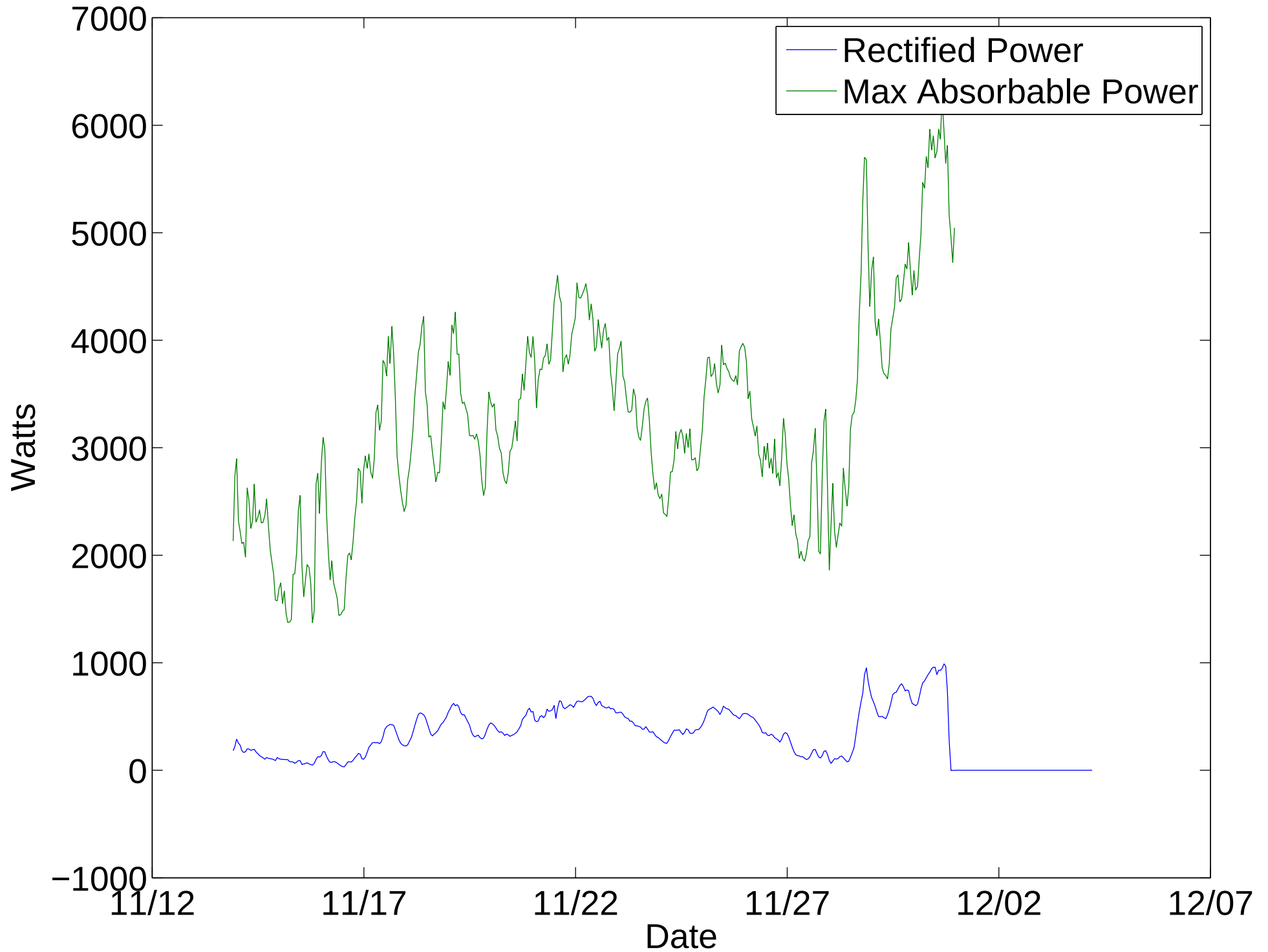
Electrical Power for Nov 13, 2012 through Nov 30, 2012
