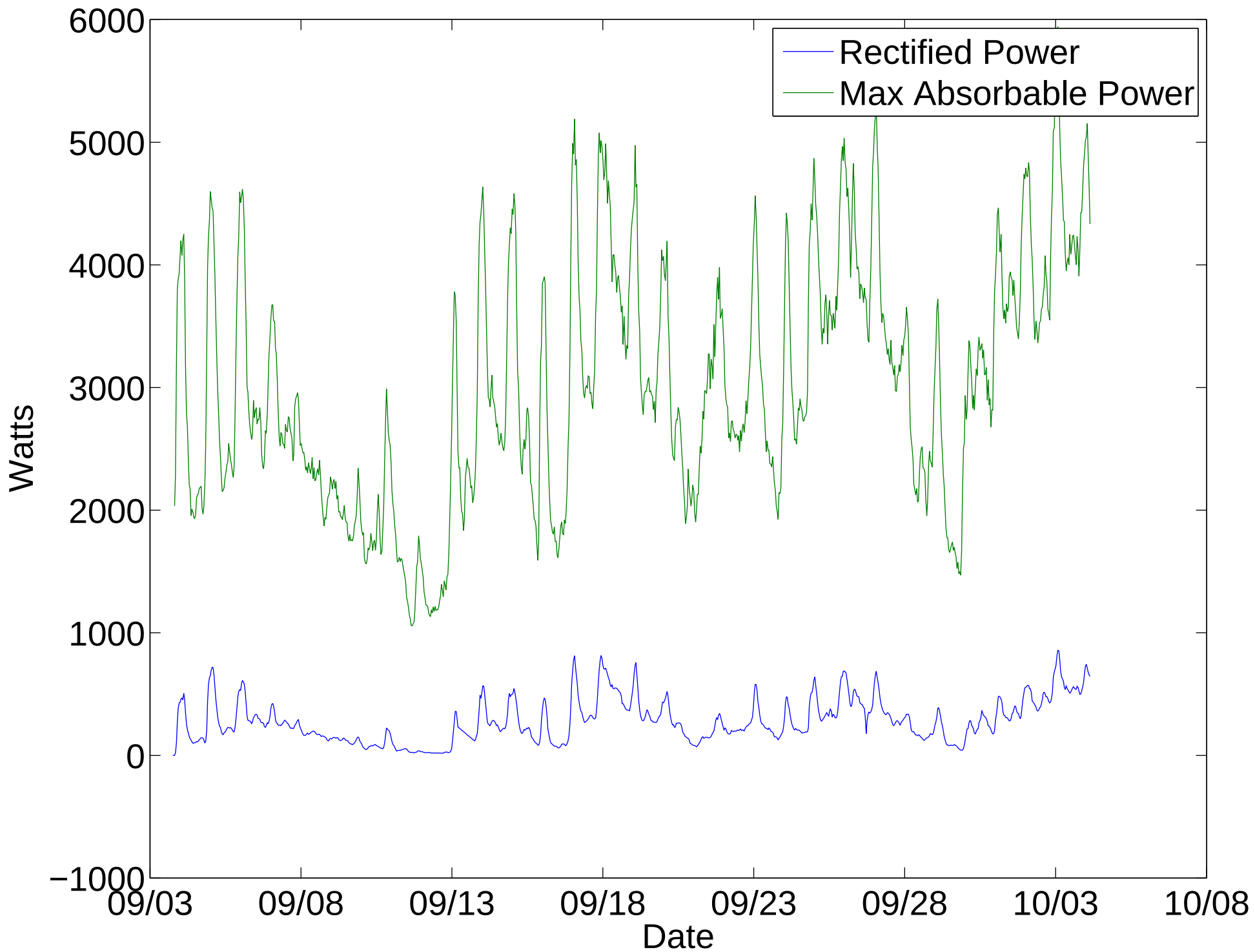
Electrical Power for 03-Sep-2013 18:04:16 through 04-Oct-2013 03:19:55
