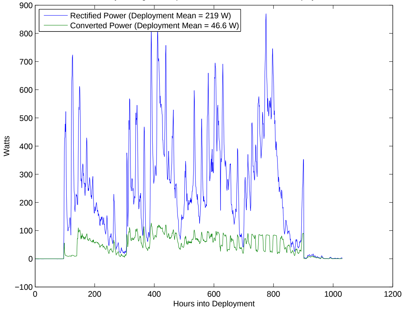
Hourly Averages of Captured Electrical Power – Entire Deployment
