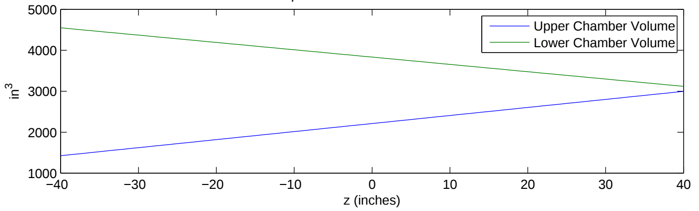
Adiabatic Compression of Diatomic Gas k = 1.675 lbs/m
