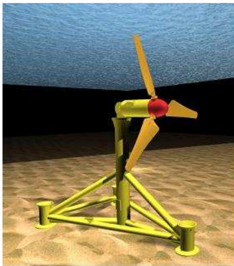
Figure 1: Fully submerged turbine initially developed by TGL and free hinge configuration at optimal speed
