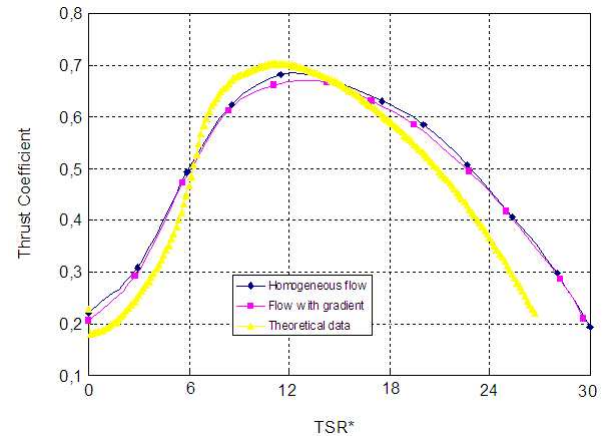
Figure 5: Thrust coefficient comparison (theoretical and experimental data) at a mean speed of 0.79 m/s
