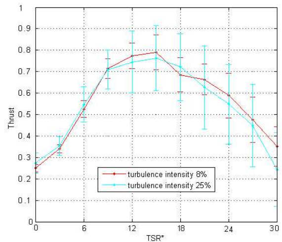
Figure 13: Normalised thrust for turbulence intensity levels of 8% and 25% at a mid-depth location
