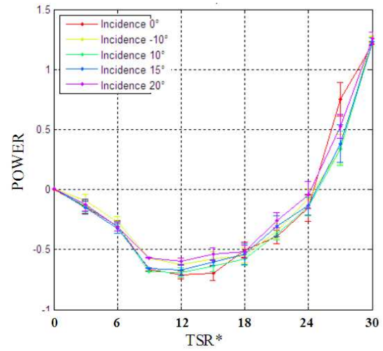
Figure 12: Measured power for several turbine orientations at a mid-depth location
