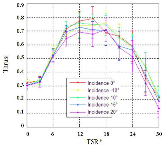
Figure 10: Normalised thrust for several turbine orientations at a mid-depth location
