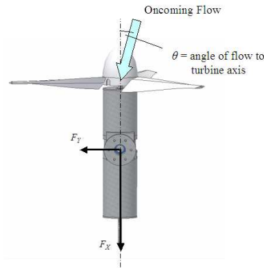
Figure 9: Scheme of the turbine orientation in the tank
