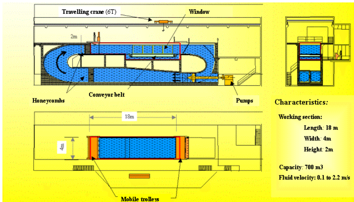
Figure 3: Ifremer free surface hydrodynamic water tunnel located in Boulogne-sur-Mer, France.
