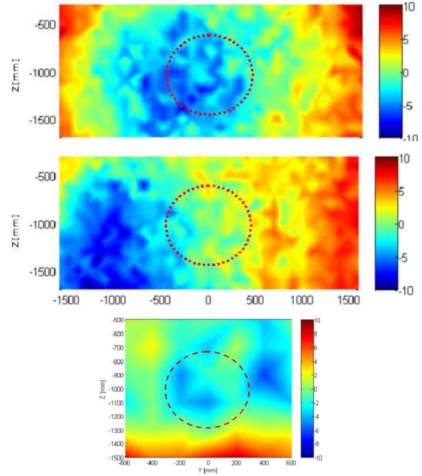
Figure 4: Maps of the flow with a mean speed of 0.79m/s for the three kinds of tested flow: homogeneous flow at the top, flow with transverse gradient of 8% at the middle and a flow with a turbulence intensity rate of ~25% at the bottom
