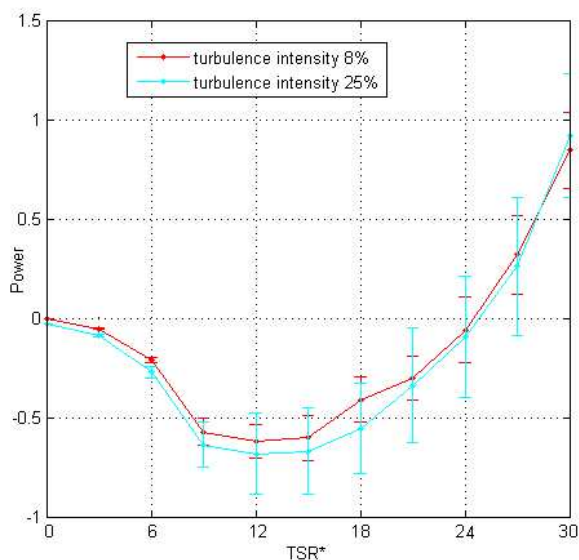
Figure 15: Measured power for both turbulence intensity rates of 8% and 25% at a mid-depth location
