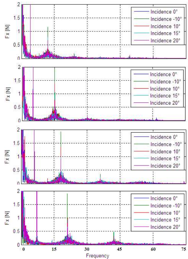
Figure 8: Axial forces spectrum for four rotor speeds for five orientation angles of the turbine in the flow between -10 to 20 degrees (increasing TSR from the top to the bottom)
