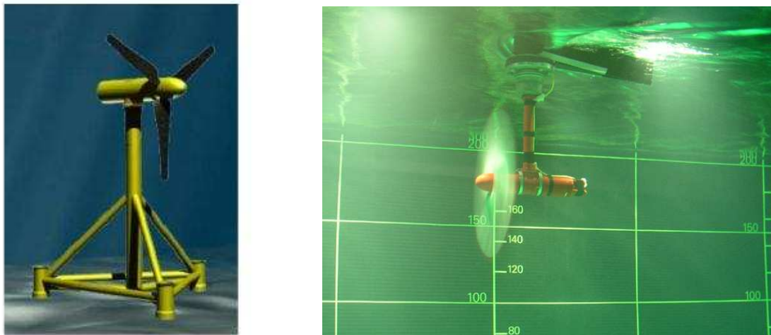
Figure 2: Fully submerged turbine now developed by TGL and model turbine during trials in the Ifremer tank
