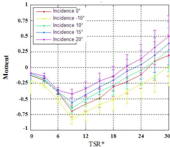
Figure 11: Normalised rotor torque for several turbine orientations at a mid-depth location
