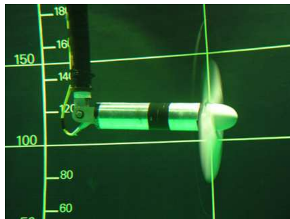
Figure 1: Fully submerged turbine initially developed by TGL and free hinge configuration at optimal speed
