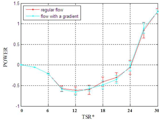
Figure 6: Measured power for an homogeneous flow and a flow with a gradient
