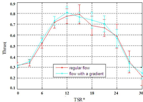
Figure 7: Normalised thrust for an homogeneous flow and a flow with a left to right gradient
