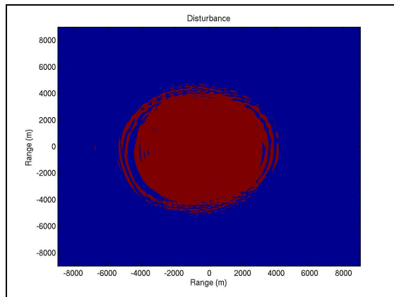
Figure 12: Case B - Zone of behavioral disturbance, considering every point with an SPL of more than 120 dB.
