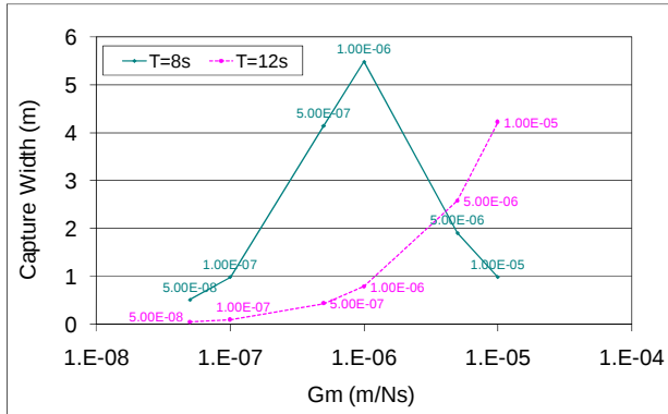
Figure 15: Capture width values obtained for different G_m parameter values (1 pair of cylinders is considered) and incident regular waves with amplitude of 1m and periods of 8 and 12s.
