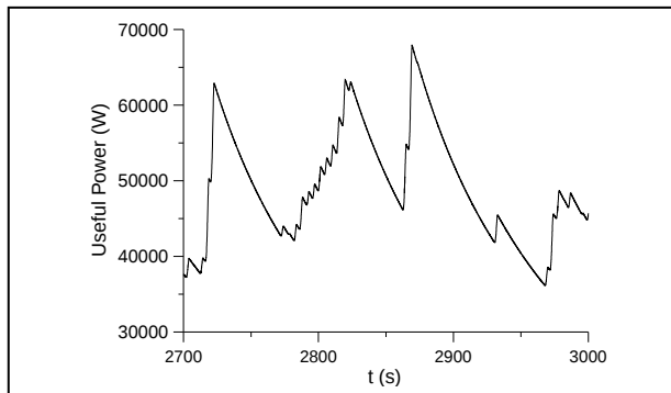
Figure 12: Useful power for significant wave height H_s = 2 m and wave energy period T_e = 8 s, assuming a non-linear power take-off mechanism with 1 pair of cylinders and G_m = 9.00E-08 m/Ns.
