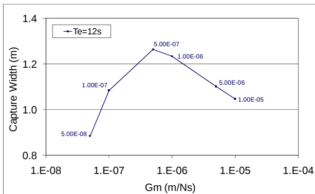
Figure 16: Capture width values obtained for different G_m parameter values (1 pair of cylinders is considered) and irregular waves with H_s = 2m and T_e = 12s .
