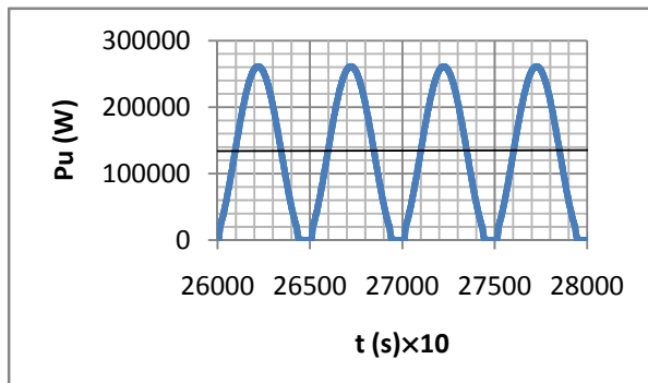
Figure 17: Useful power values obtained for test 2, T=10.05 s and 1m wave amplitude.
