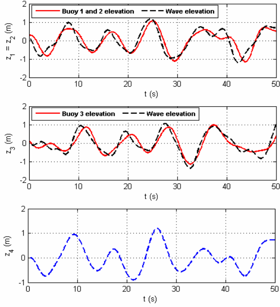
Fig. 4. Heave oscillations of buoys 1, 2 and 3 and body 4. Irregular waves of H_s = 2\text{ m} , T_e = 10\text{ s} , \beta = 30^\circ , \theta = 0 .
