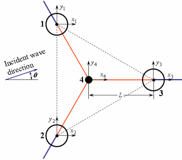
Fig. 1. Plan view of buoys 1 to 3, weight 4 and mooring lines in calm-sea static conditions. The wave direction makes an angle \theta with the x -axes.
