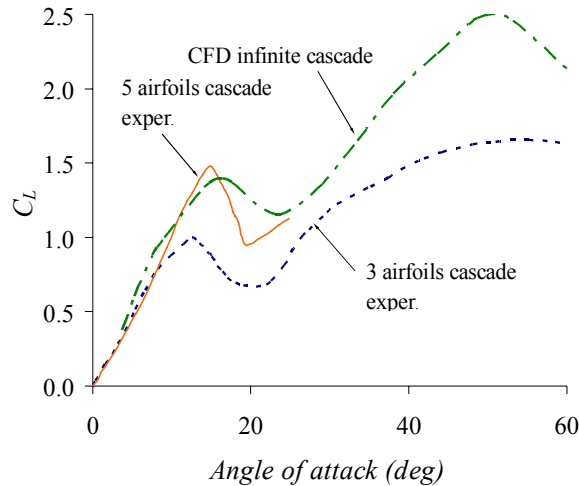
Figure 9: Comparison of experimental data for cascades of three and five NACA0021 aerofoils [10] with a CFD simulation from the present work for an infinite cascade ( \sigma = 0.5 )
