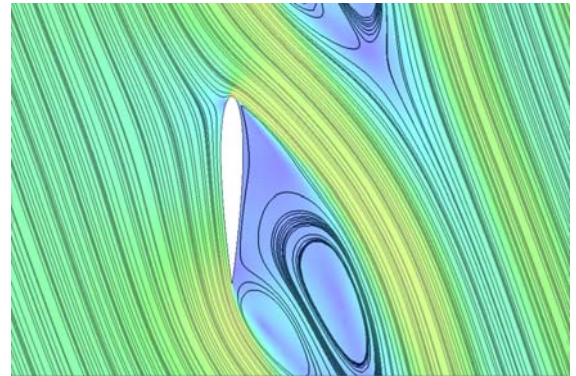
Figure 5: CFD prediction of streamlines in a tandem cascade ( \gamma = 0^\circ ) with s/c = 2 and \alpha_m = 20^\circ .
