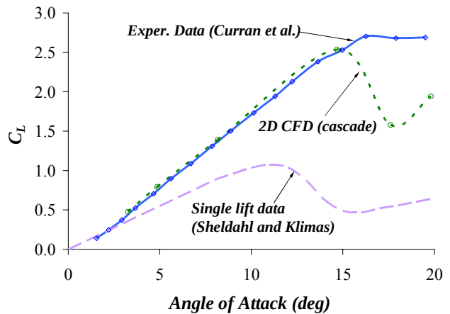
Figure 10: Comparison of lift coefficients deduced from CFD analysis and experimental rotor tests [13] for a Wells monoplane turbine with NACA0012 blade profile ( \sigma=0.64 ). Isolated aerofoil lift data are also provided [14].
