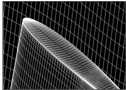
Figure 13: Typical example of a structured mesh on the blade surface for \gamma = 32^\circ .
