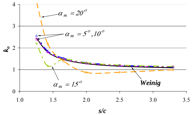
Figure 4: Lift coefficient interference factor ( k_0 ) for a linear tandem cascade ( \gamma = 0^\circ ) of NACA0012 aerofoils as a function of s/c and the mean angle of incidence, \alpha_m : \square 5^\circ ; \Delta 10^\circ ; \diamond 15^\circ ; \circ 20^\circ . Broken lines - CFD analysis; solid line - Weinig's inviscid flow analysis, eqn. (2).
