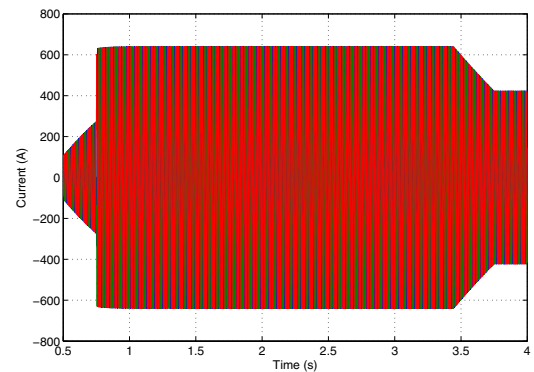
Figure 10: Grid current during LVRT event
