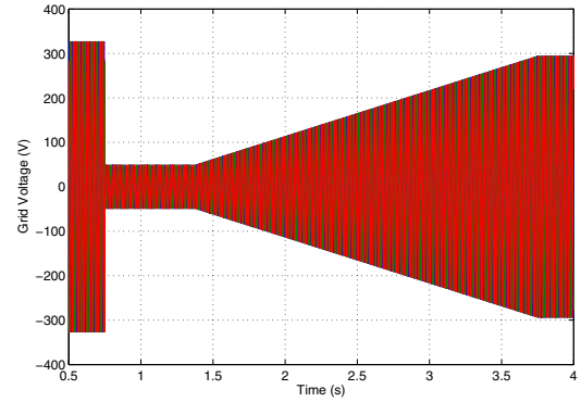
Figure 9: Grid voltage during LVRT event
