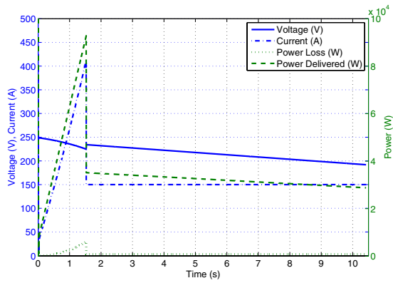
Figure 8: Supercapacitor voltage, current, power, and power loss during turbine start-up
