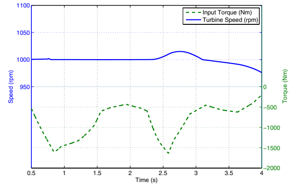
Figure 13: Turbine speed and input torque during LVRT event with supercapacitors
