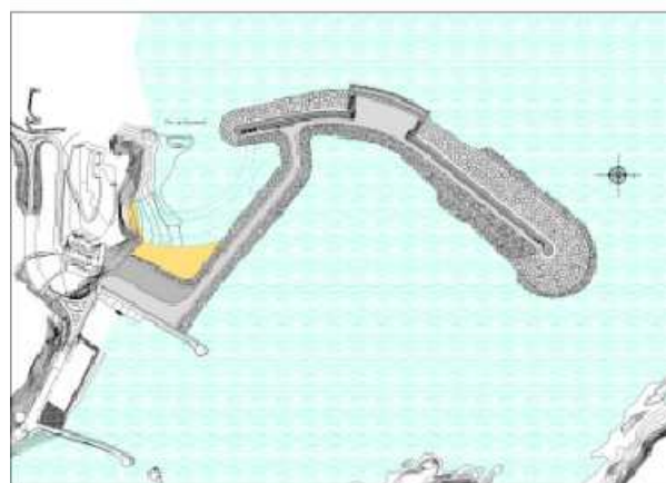
Figure 7. Plan of the arrangement with the OWC plant.
