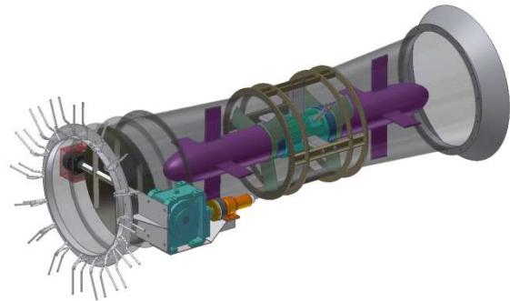
Figure 5. Wells turbine tested at LIMPET.
