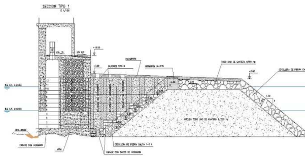
Figure 8. Section at the OWC plant.
