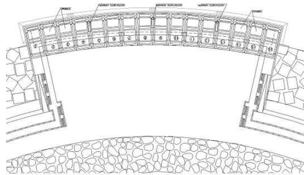
Figure 10. Plan of the OWC plant.
