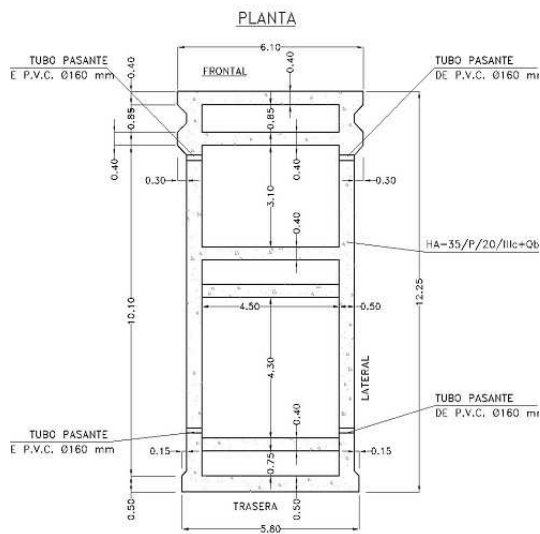
Figure 9. Prefabricated part to build the caissons.
