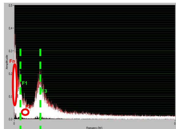
Figure 7: FFTs of CoRMaT pitch data showing the dominant frequencies at Islay.
