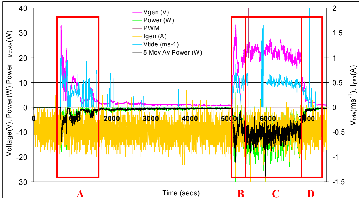
Figure 4: CoRMaT operational overview at Sound of Islay
