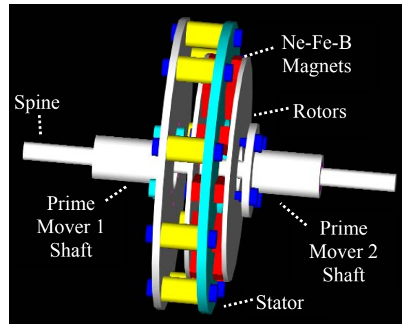
Figure 9: CAD rendering of contra-rotating axial flux generator.
