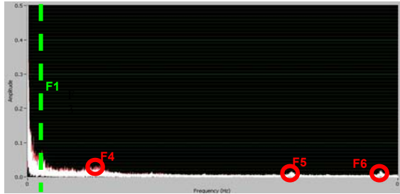
Figure 8: FFTs of CoRMaT roll data showing the dominant frequencies at Islay.
