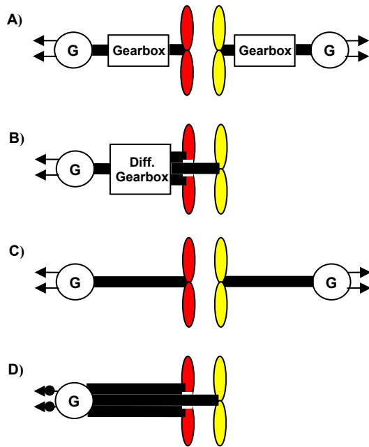
Figure 10: Power Take-off Options
