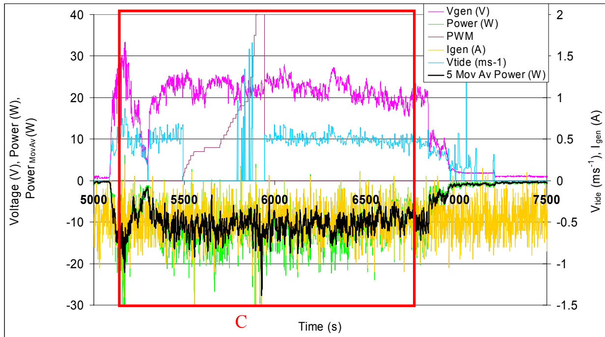
Figure 5: CoRMaT operation at Sound of Islay test site.
