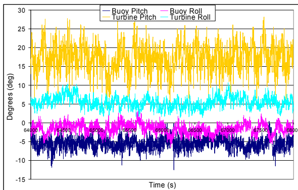
Figure 6: Example of turbine and surface buoy inclinometer data.
