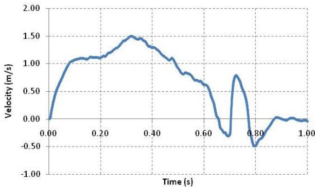
Figure 8 –Velocity of a cylinder submerged 0.5m below the free surface and allowed to rise to equilibrium point
