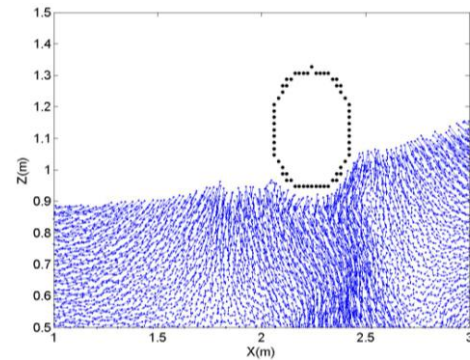
Figure 10 – Velocity plots of the fluid domain as the incoming wave reaches the floating object. The frames are separated by t=0.3 seconds.
