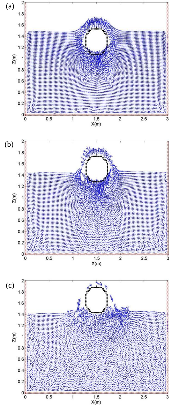
Figure 9 – Velocity plots of the fluid domain as the cylinder rises through the fluid (a), breaches the surface (b), and as the cylinder comes to rest (c).
