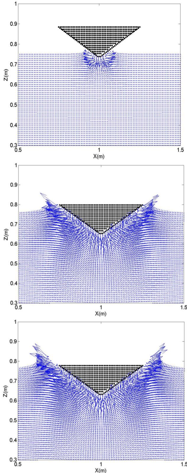
Figure 3. The velocity plot for the fluid domain at times 0.004s, 0.016s and 0.02s. The jets as described in Greenhow [23] can be clearly seen.
