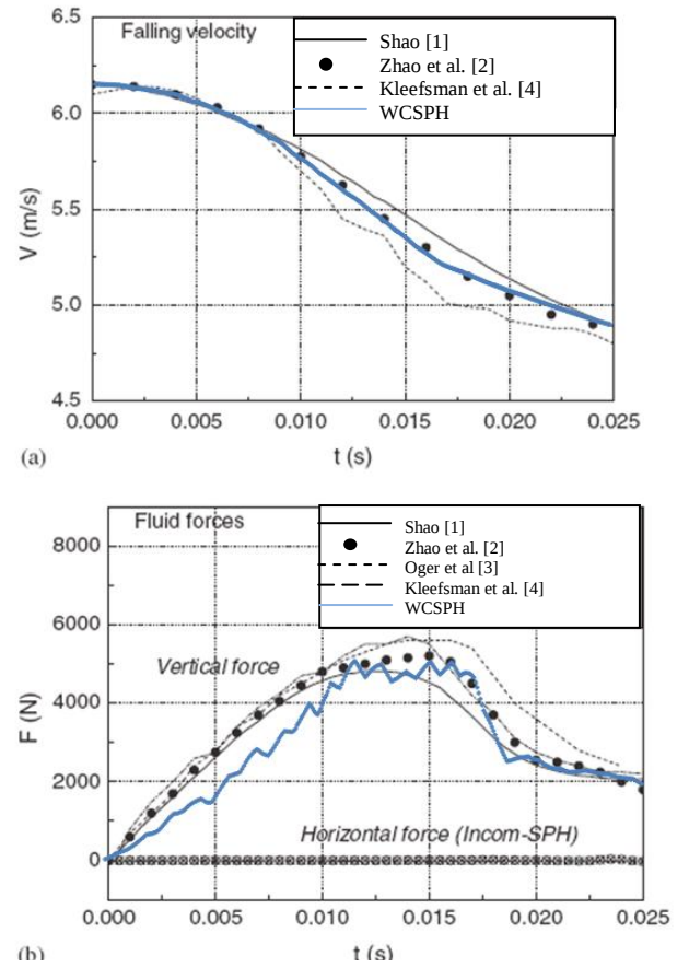
Figure 2. (a) The falling velocity of a wedge with a 30^\circ dead rise angle, timed from the moment of initial impact. (b) The vertical force exerted on the wedge by the fluid body. Authors results (WCSPH) in blue plotted on graph from [23]
