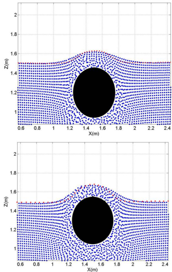
Figure 6 - Free surface deformation due to a cylinder rising through the free surface, for dimensionless time ( T=Ut/d ) of 0.4 and 0.6. Red dots show the numerical results presented in Greenhow and Moyo [27]
