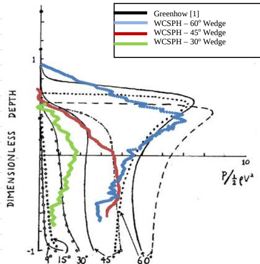
Figure 5 – Slamming coefficient against dimensionless depth for 2D wedges plotted over the predicted values from Greenhow [23]
