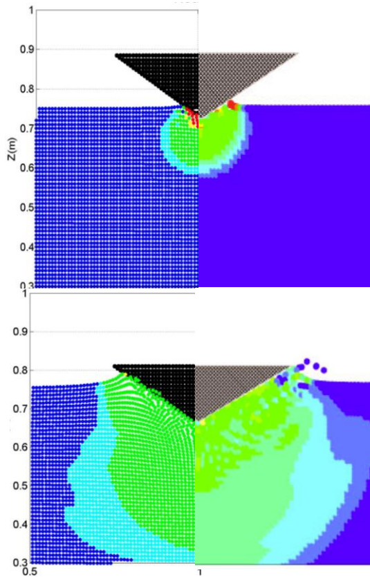
Figure 4 –Pressure under the impact of the wedge with weakly compressible SPH on the left hand side and the results of Shao[1] on the right.
