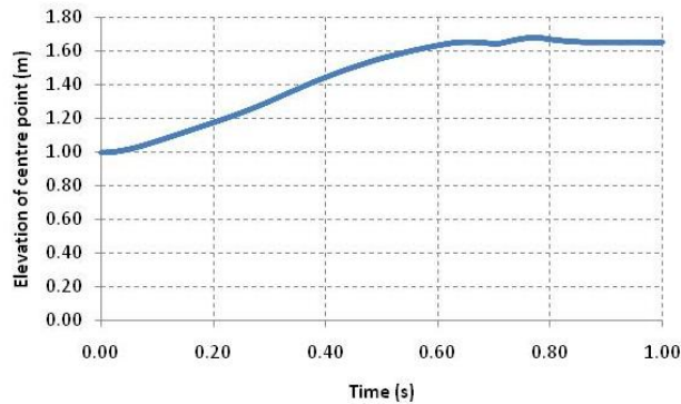
Figure 7 – Elevation of a cylinder submerged 0.5m below the free surface and allowed to rise to equilibrium point
