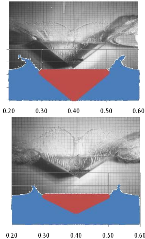
Figure 1: Comparison of SPH (colour) and the results of Greenhow (black and white) for a controlled plunging of a wedge with a 45^\circ (top) and a 30^\circ (bottom) deadrise angle.
