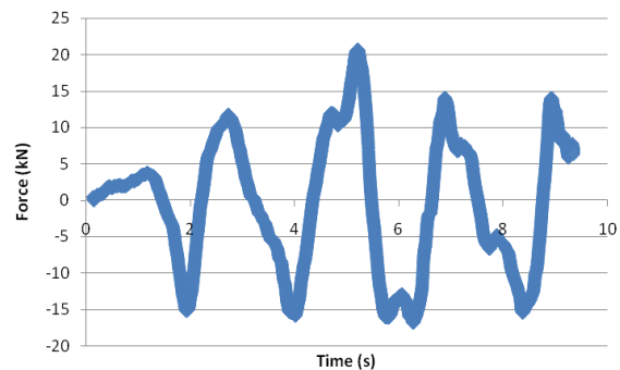
Figure 11 – Lateral hydrodynamic forcing on the cylinder over several typical wave cycles.
